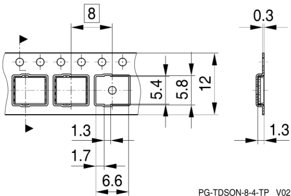
PG-TDSON-8-4-TP V02
