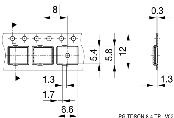
PG-TDSON-8-4-TP V02
