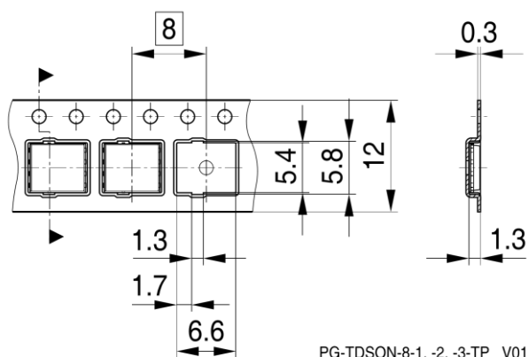
PG-TDSON-8-1, -2, -3-TP V01
