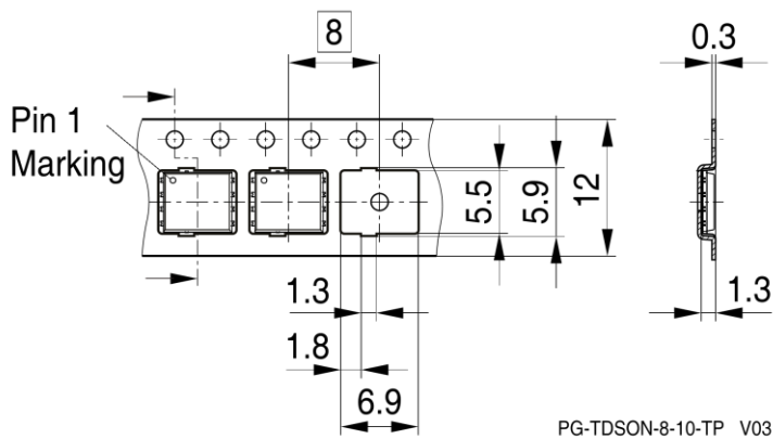
PG-TDSON-8-10-TP V03
