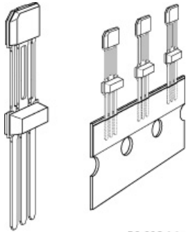
PG-SSO-3-9x
