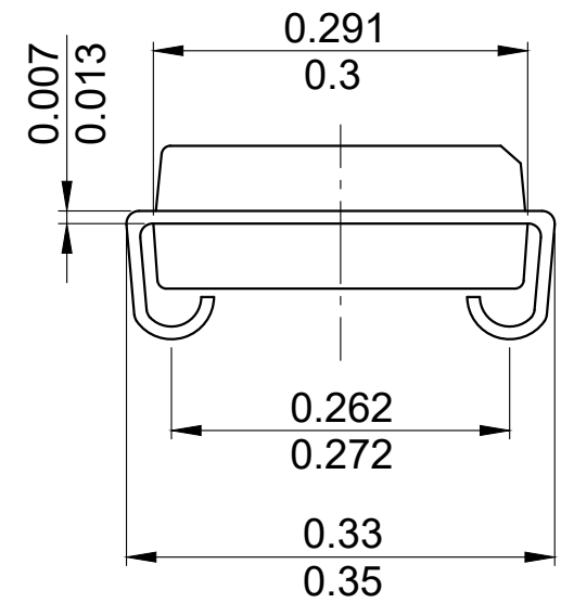
Detail A External lead design
