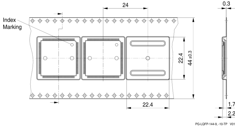
PG-LQFP-144-9, -10-TP V01
