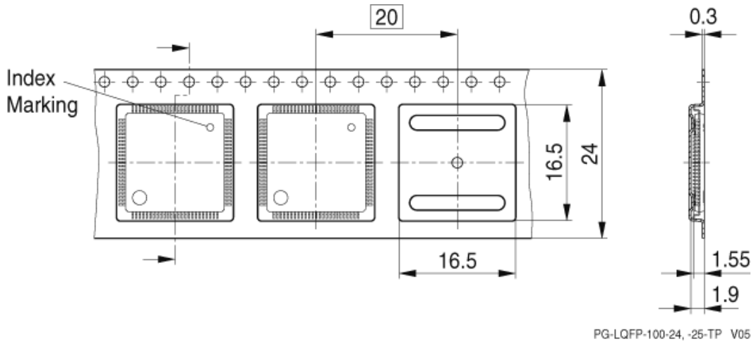
PG-LQFP-100-24, -25-TP V05
