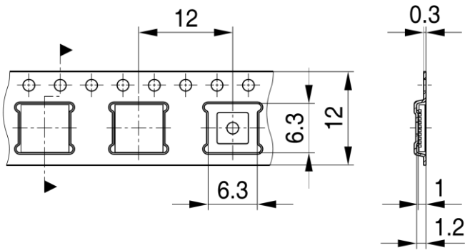
PG-IQFN-40-1-TP V01
