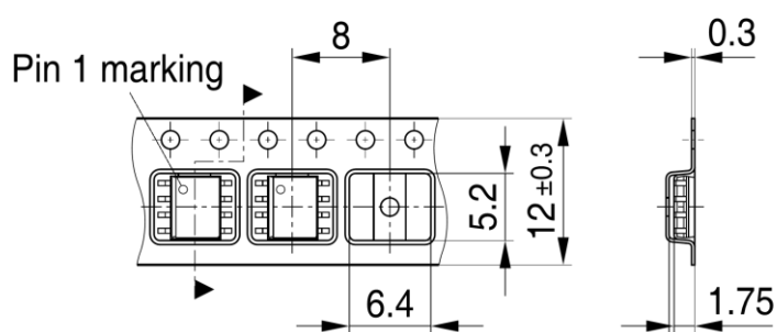
PG-DSO-8-27-TP V05
