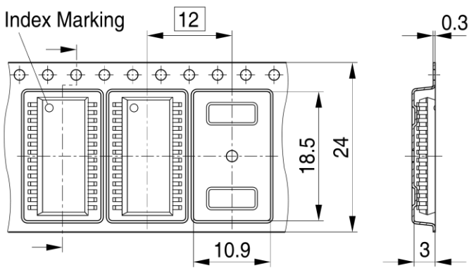
PG-DSO-28-1-6-7-9-11-13-14-16-to-19-21-to-24-26-27-29-to-36-38-41-to-45-73-TP V07
