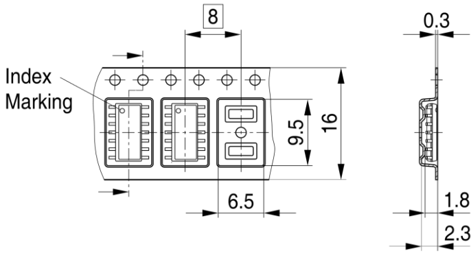
PG-DSO-14-33, -40, -43, -47, -48-TP V01
