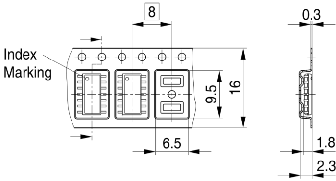
PG-DSO-14-33, -40, -43, -47, -48-TP V01
