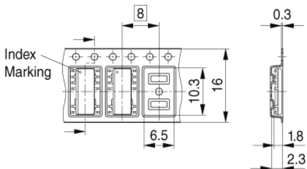
PG-DSO-12-19, -20-TP V07
