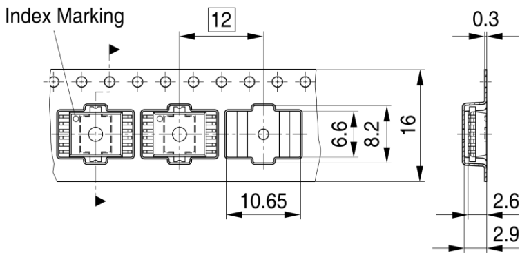
PG-DSO-12-4, -5, -8, -11, -12, -16-TP
