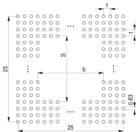
PG-BGA-416-4, -10, -13, -14-FP W01
