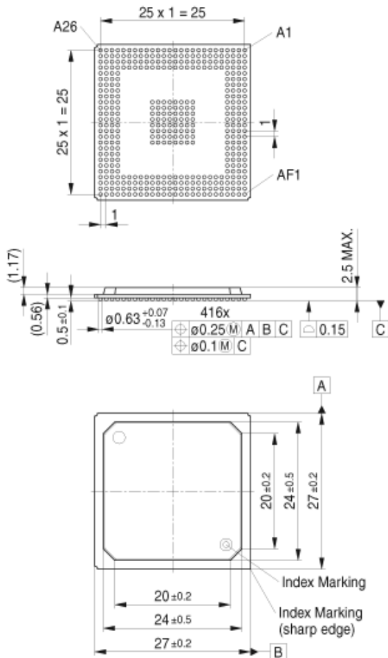
PG-BGA-416-4, -10, -13, -14-PO W06
