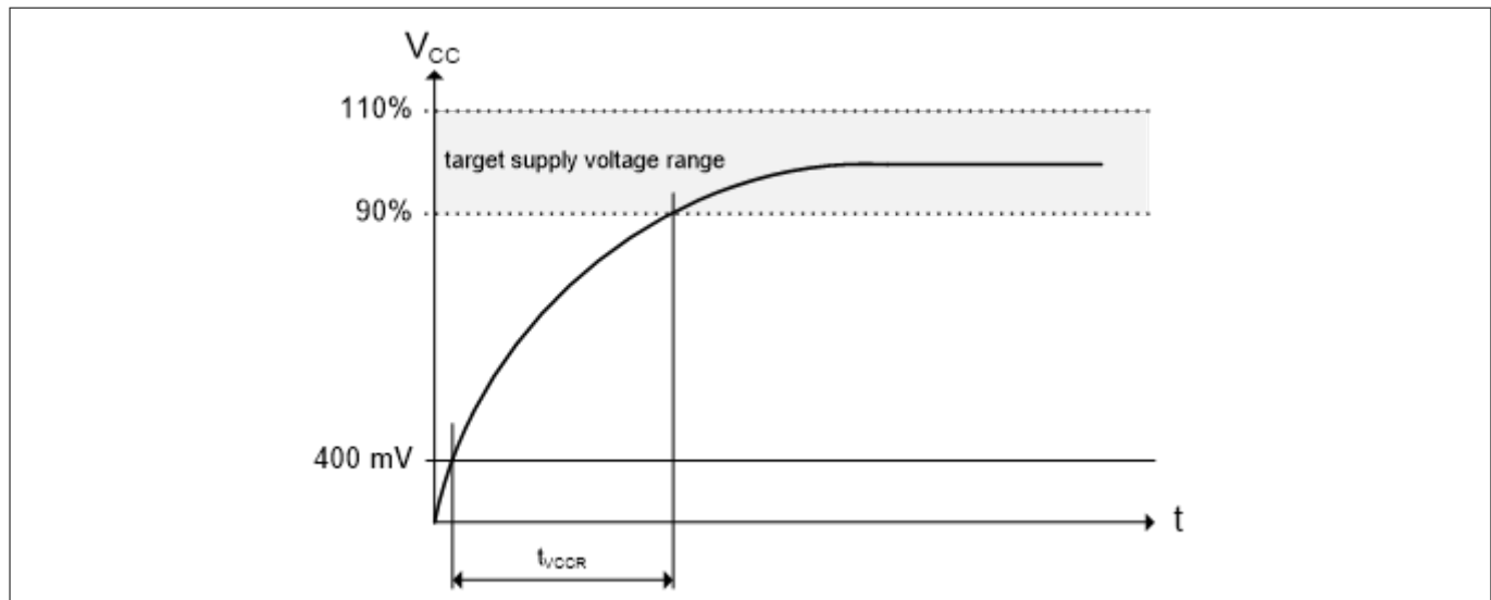
Figure 9 V_{CC} rampup
