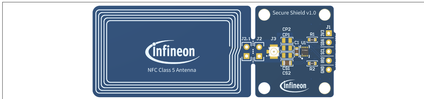
The OPTIGA™ Authenticate NBT Shield, as shown in Figure 3 , provides the pin header J1 that allows to easily connect the NBT Shield to various host MCU boards (for example via the included five-pin jumper cable). Alternatively, these pins can also be connected to an adapter board, which allows it to be directly plugged into specific host boards. By default, the OPTIGA™ Authenticate NBT Shield comes with a detachable host MCU adapter board (see Chapter 2.4 ).
