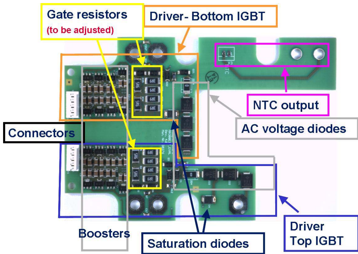
Figure 7 The MA300E12 with marked functions
