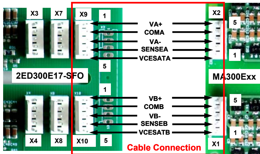
Figure 5 Connections between 2ED300E17-SFO and MA300Exx
