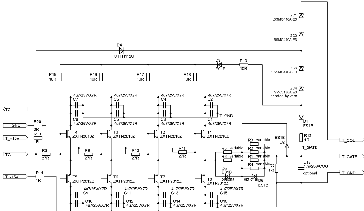
Figure 13 The MA300Exx – top IGBT
