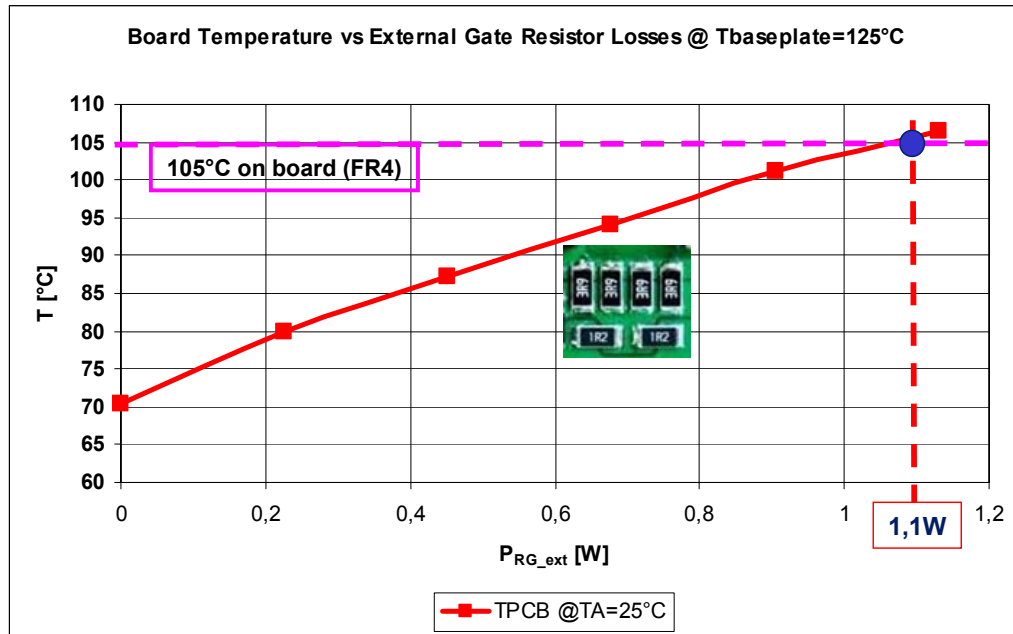
Figure 11 PCB temperature vs. gate resistor power losses
