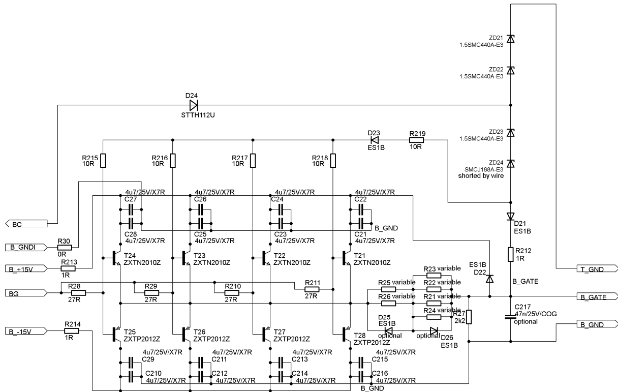
Figure 14 The MA300Exx – bottom IGBT
