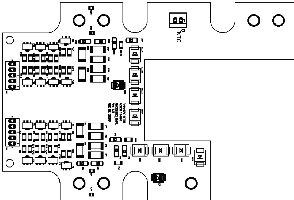
Figure 17 The MA300Exx – assembly drawing
