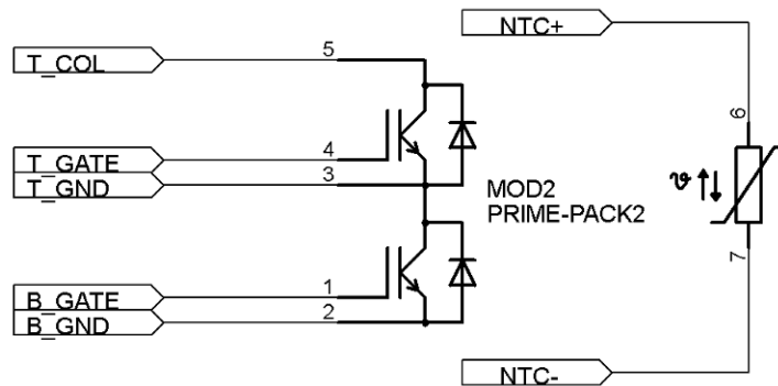
Figure 15 The MA300Exx – main connectors
