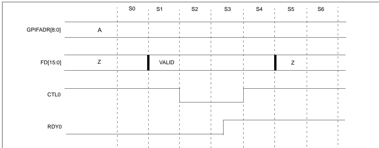
Figure 10-9. One Decision Point: No Wait States Inserted: RDY0 is Already Low at Decision Point I1
