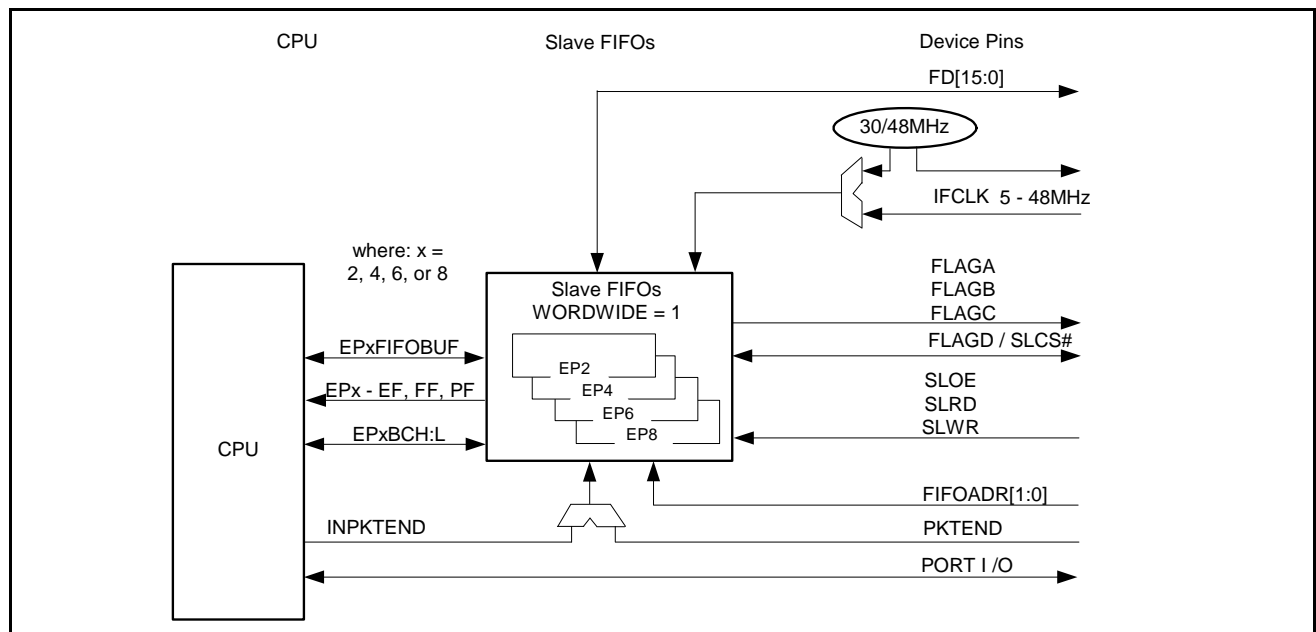
Figure 9-1. Slave FIFOs Role in the MoBL-USB FX2LP18 System
