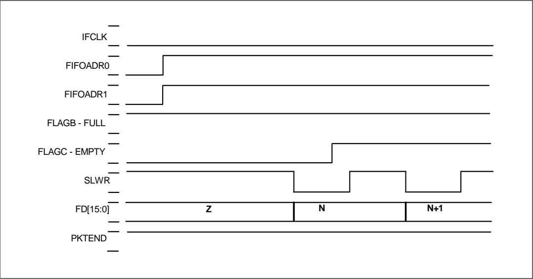
Figure 9-21. Timing Example: Asynchronous FIFO Writes
