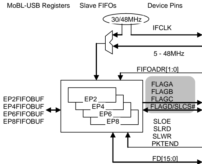
Figure 9-8. FLAGx Pins
