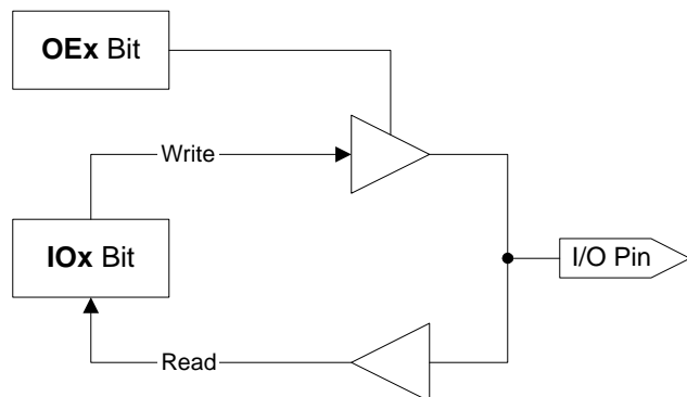
Figure 13-1. MoBL-USB FX2LP18 IO Pin
