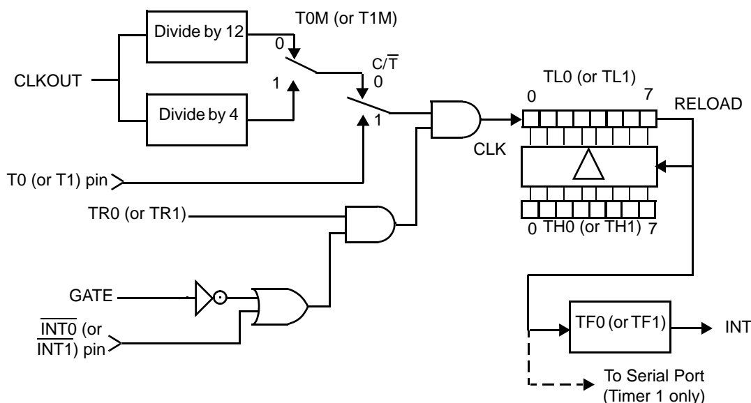
Figure 14-2. Timer 0/1 - Mode 2
