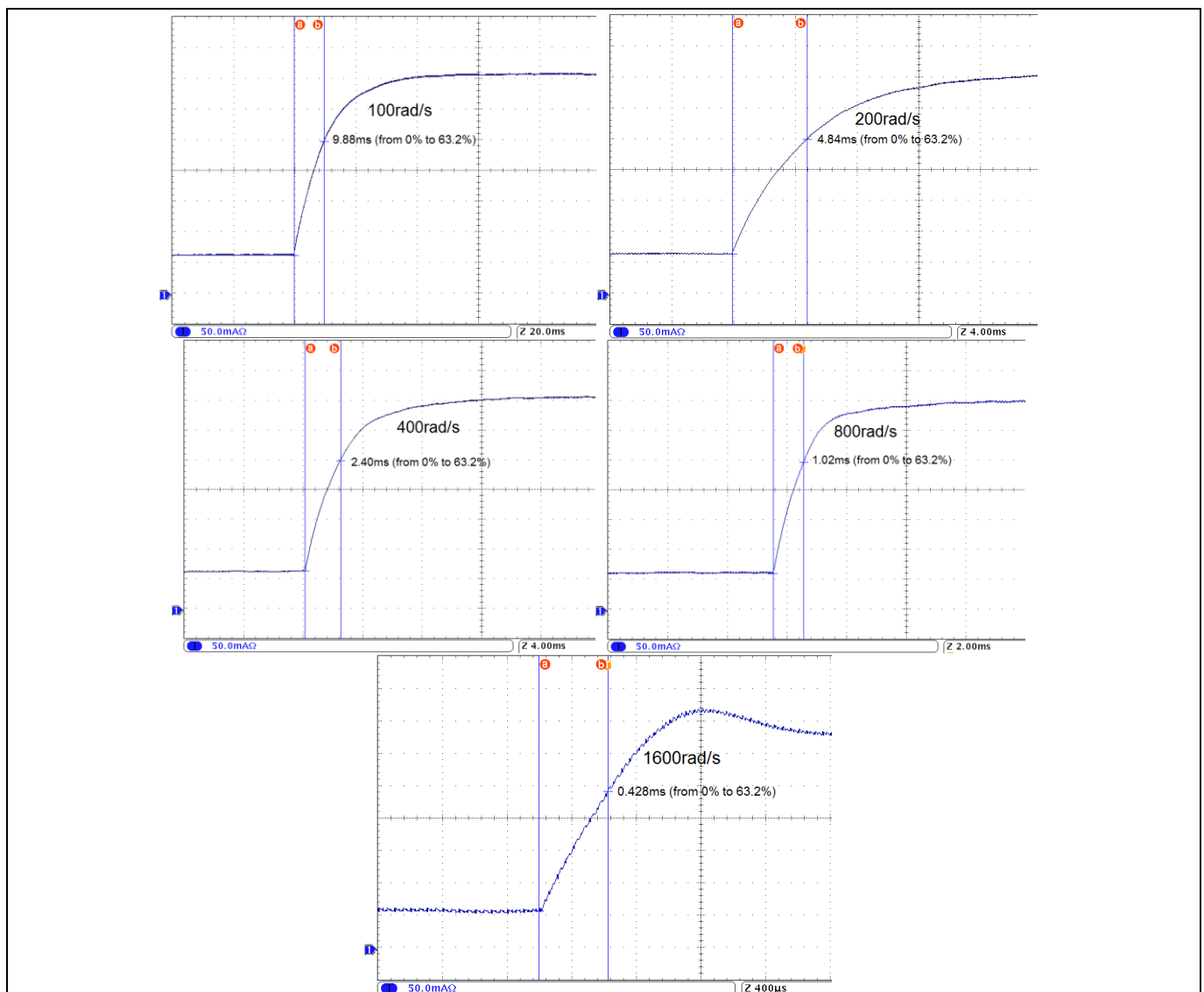
Figure 51 Current regulator step response (100/200/400/800/1600rad/s)
