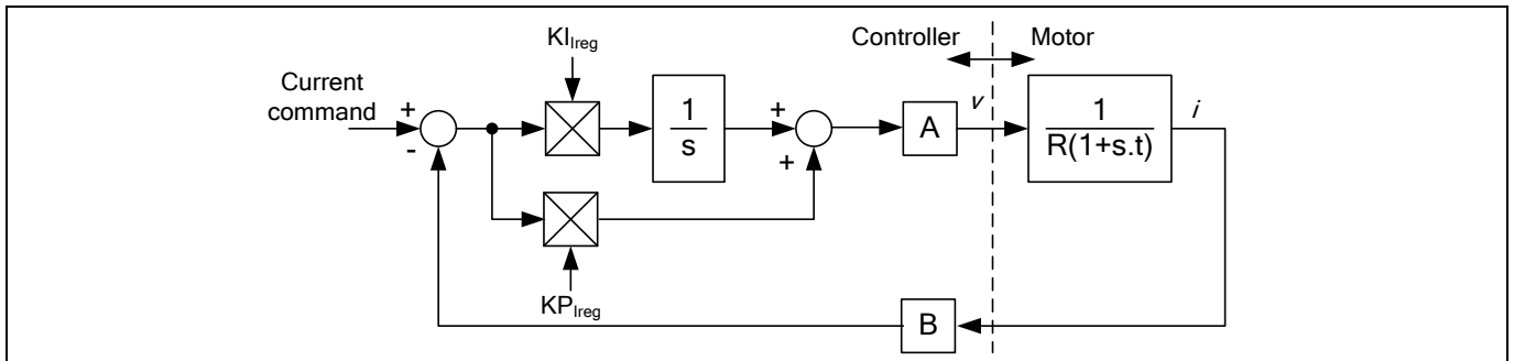
Figure 48 Current controller dynamics
