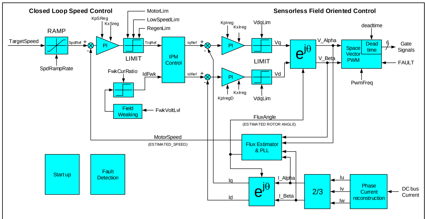
Figure 1 Top level diagram of speed control loop and sensorless FOC
