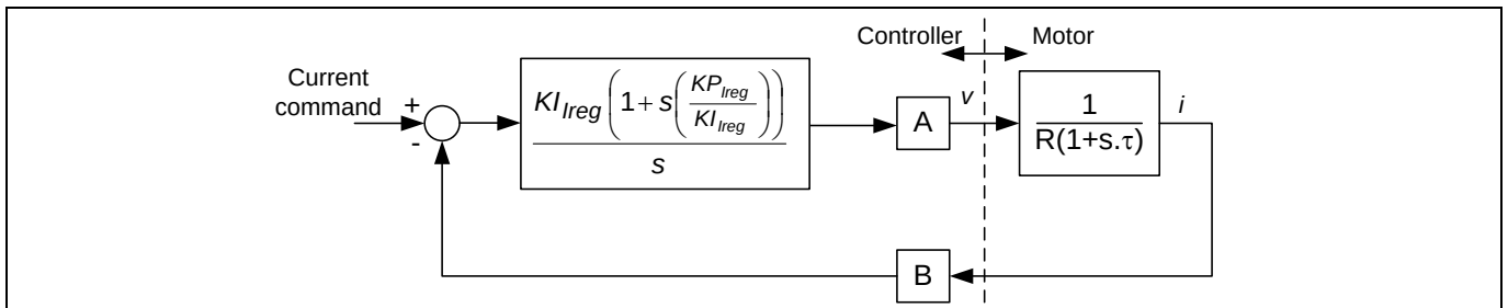
Figure 49 Pole zero cancellation
