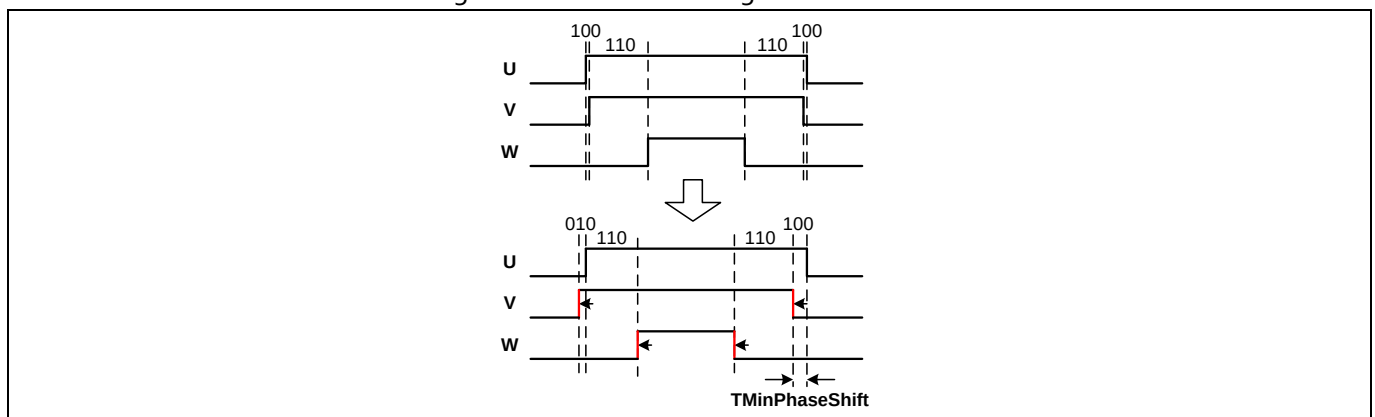
Figure 39 TminphaseShift PWM
