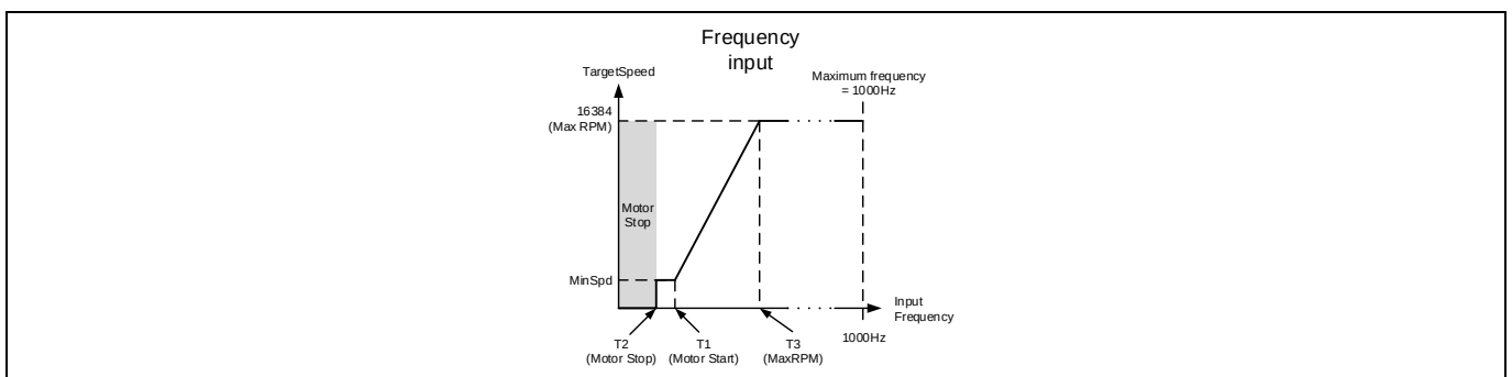
Figure 21 Frequency Input
