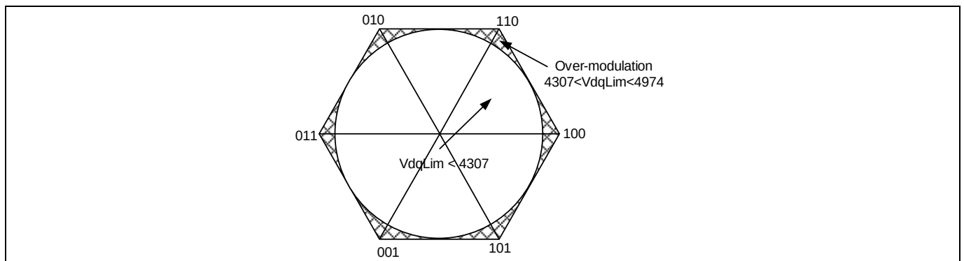
Figure 43 Over modulation
