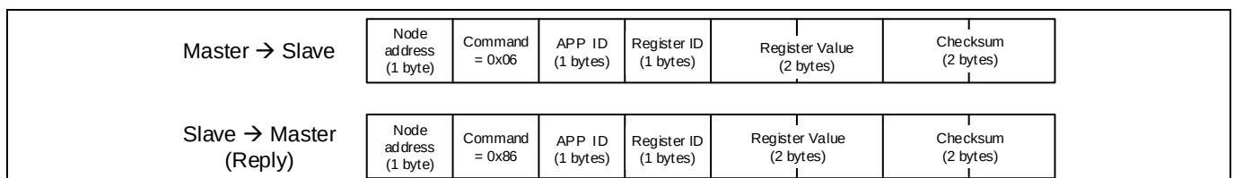
Figure 34 Register Write Command
