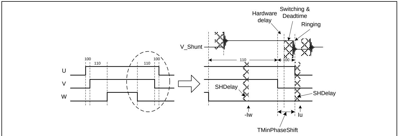
Figure 46 Single Shunt Current Sensing for Phase Shift PWM
