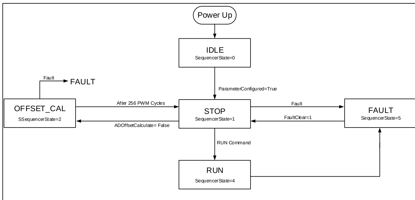
Figure 27 State handling flow chart
