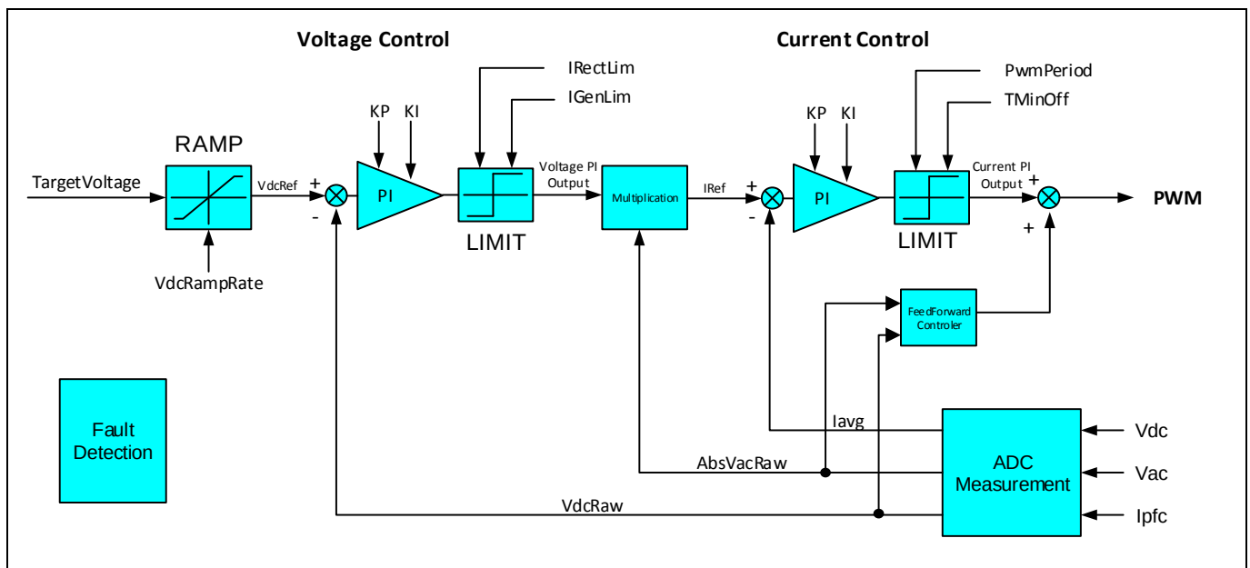
Figure 24 Top level diagram of Power Factor Correction
