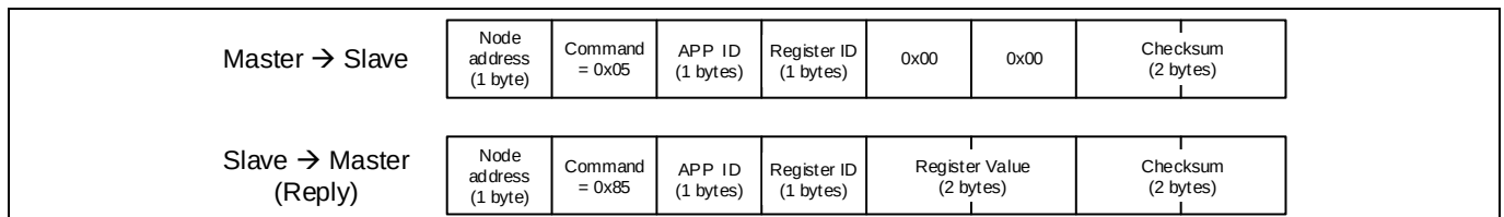
Figure 33 Register Read Command
