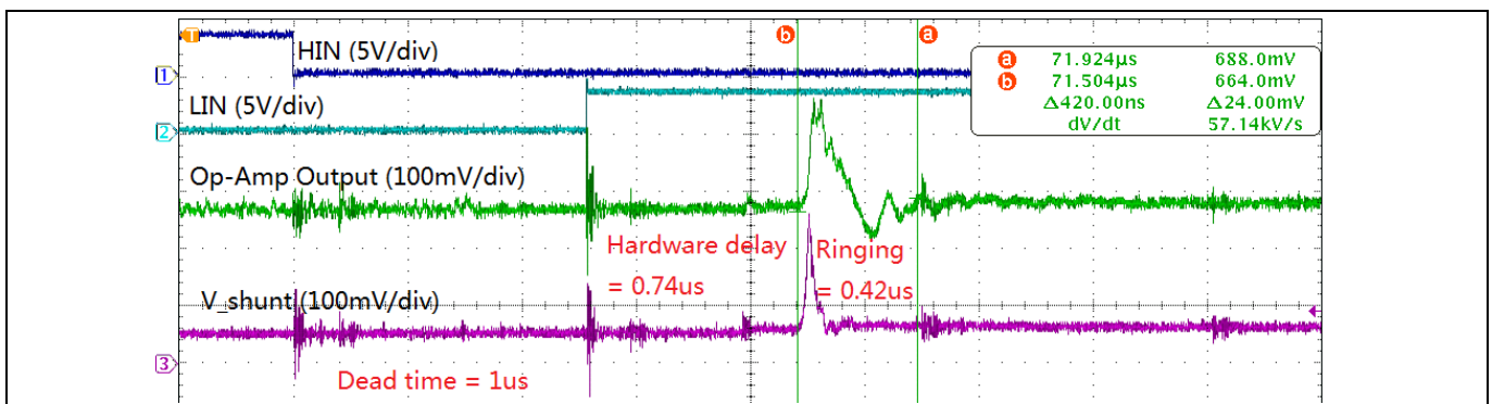
Figure 47 Measuring hardware delay and ringing time
