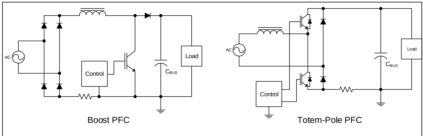
Figure 25 PFC topologies
