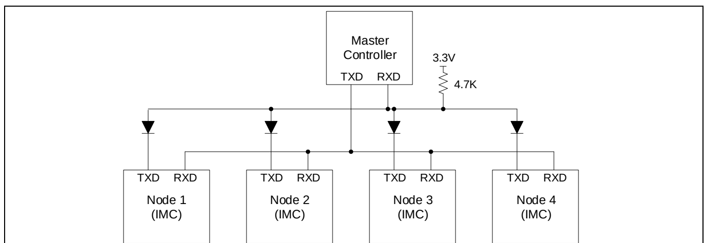
Figure 37 UART network connection
