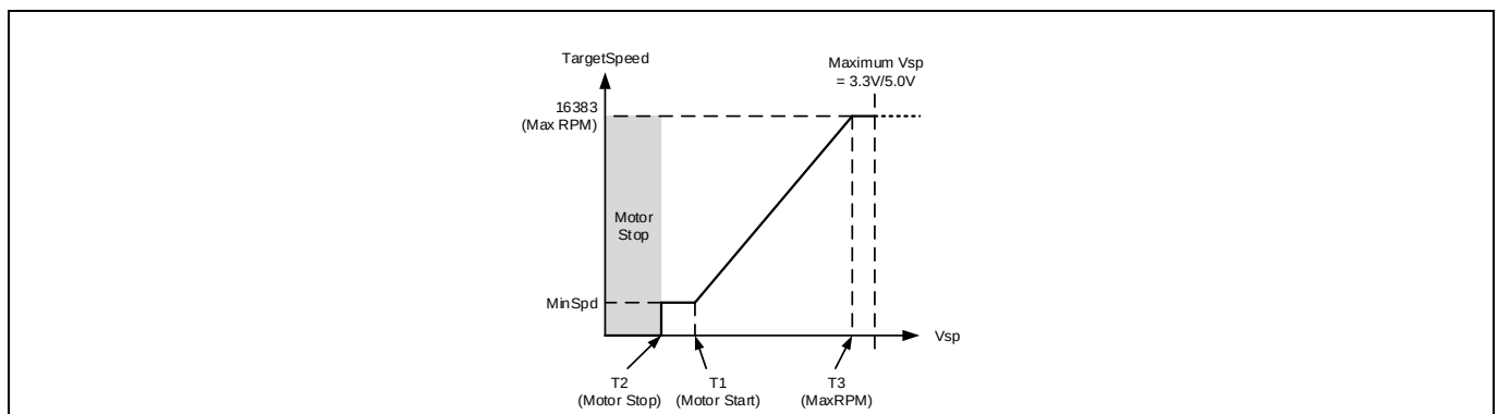
Figure 20 Vsp Analog Input
