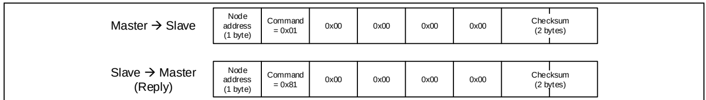
Figure 30 Clear fault command
