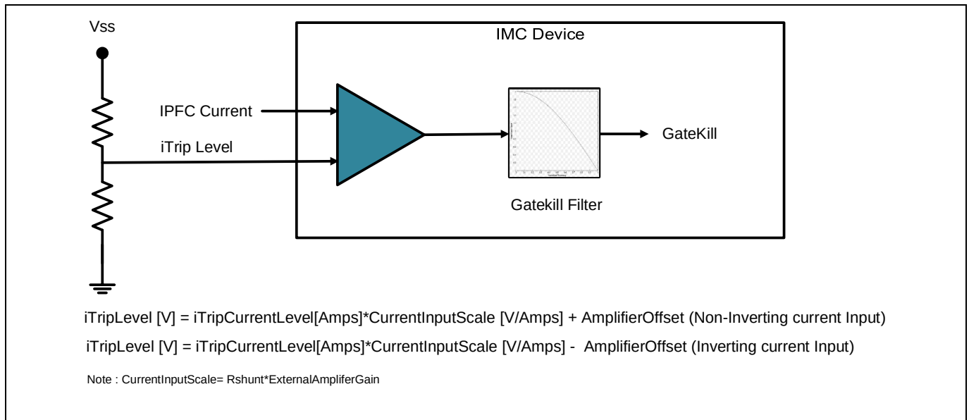
Figure 26 PFC Gatekill setup
