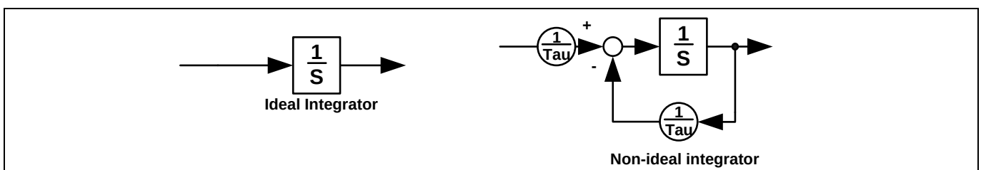
Figure 42 Ideal and Non-ideal Integrator
