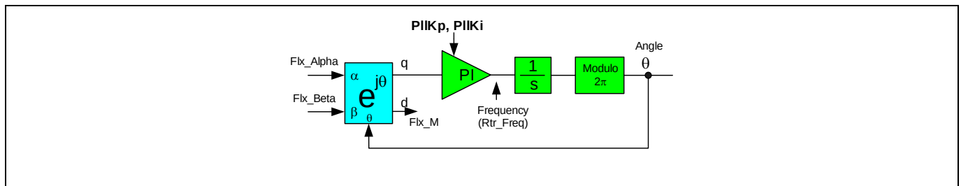
Figure 11 Simplified block diagram of a Flux PLL
