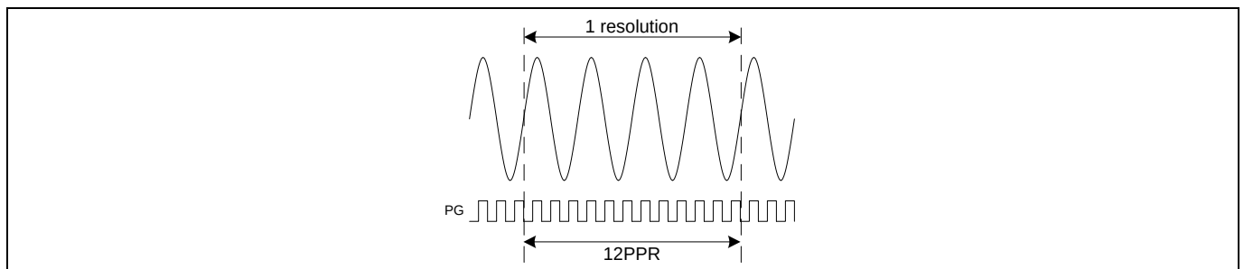
Figure 45 PG Output
