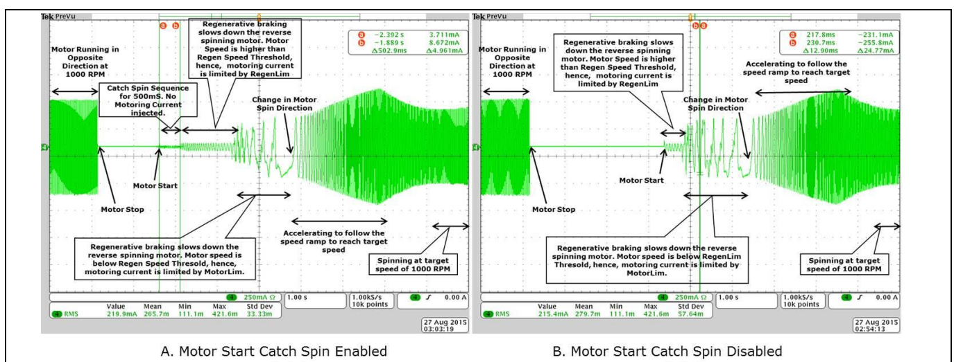
Figure 19 Motor Phase Current Waveform - Reverse Catch Spin - Motor start with/without catch spin
