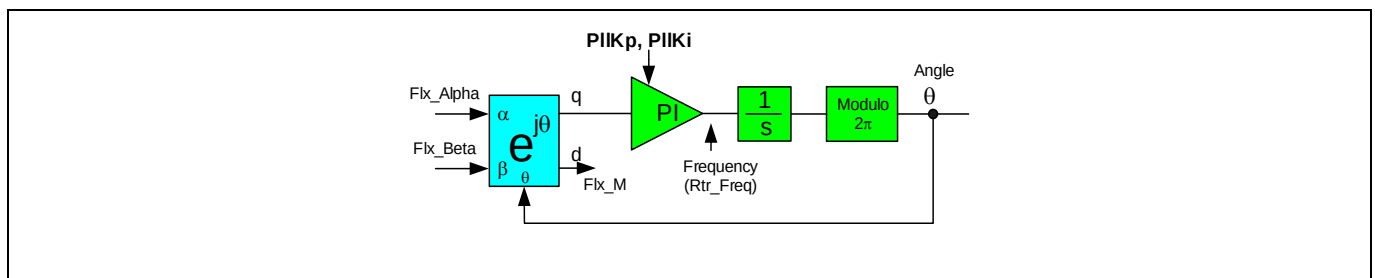
Figure 41 Simplified Block diagram of a FLUX PLL
