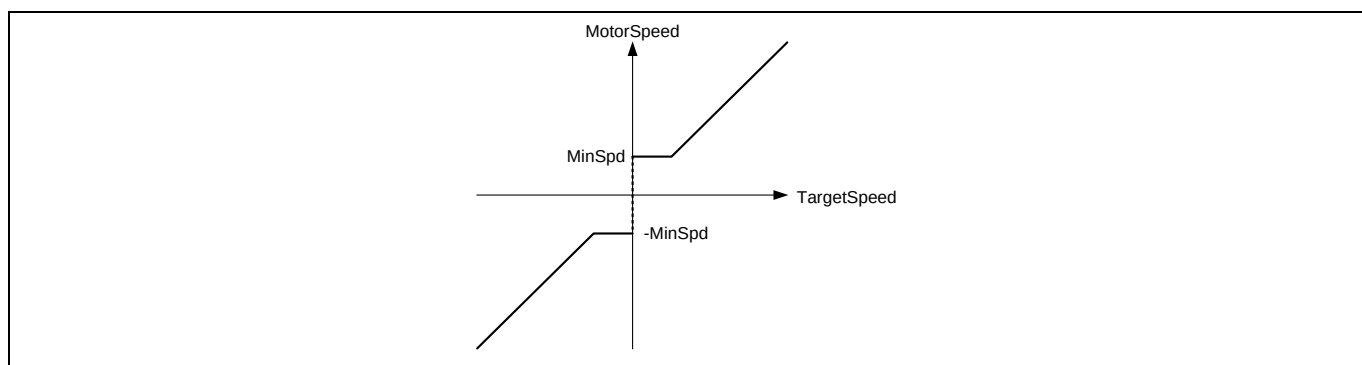
Figure 40 Minimum Speed
