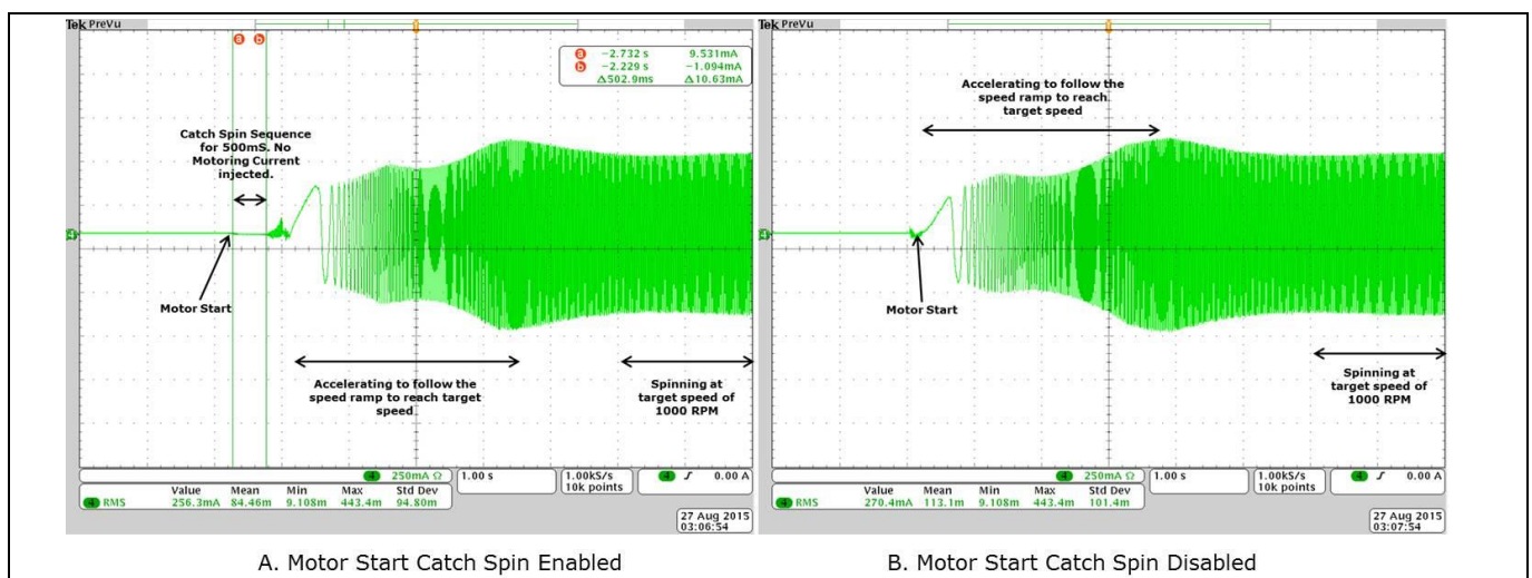
Figure 15 Motor Phase Current - Zero Speed Catch Spin - Motor start with/without catch spin
