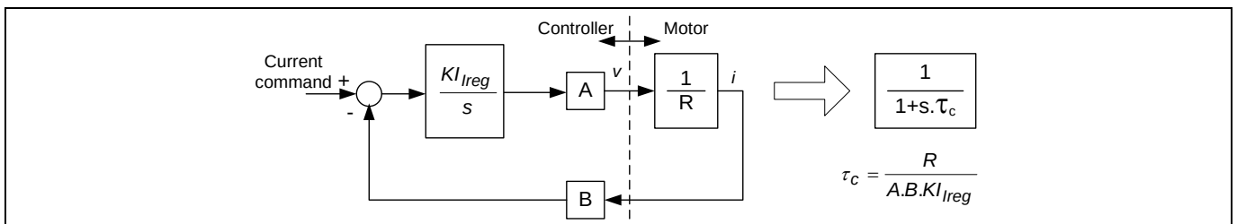
Figure 50 Simplified current control dynamics due to pole zero cancellation
