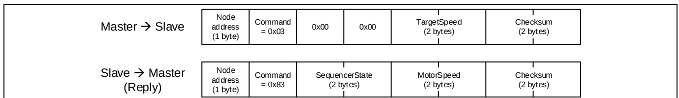
Figure 32 Motor control Command
