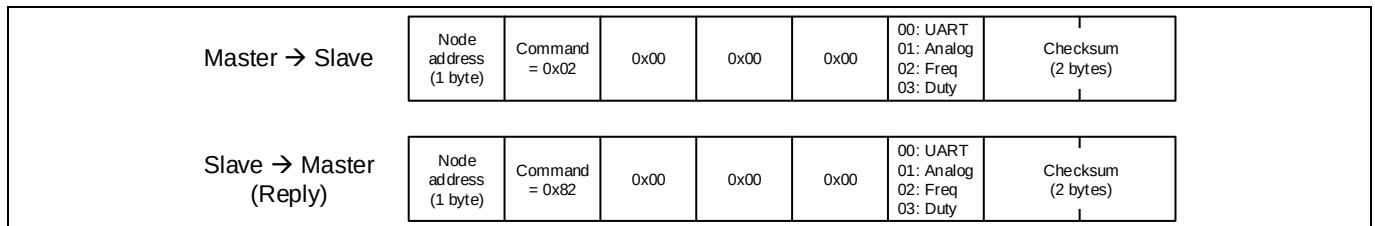
Figure 31 Control input mode command
