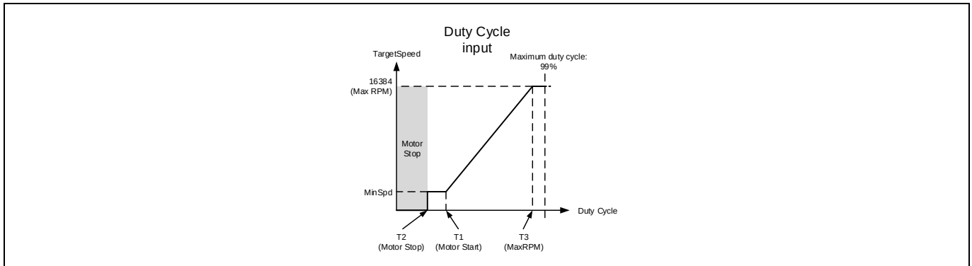
Figure 22 Duty Cycle Input
