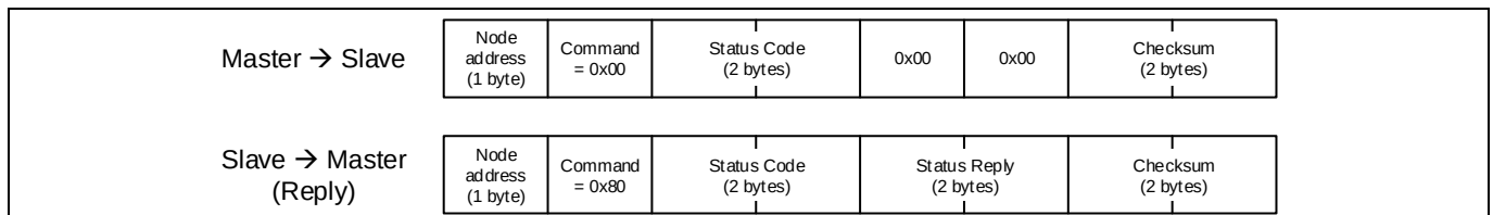
Figure 29 Read Status command
