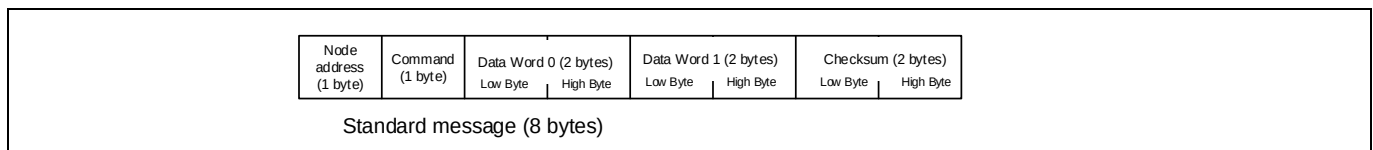
Figure 28 UART Data Frame
