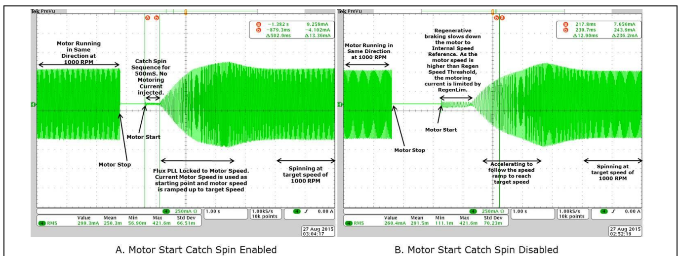
Figure 17 Motor Phase Current Waveform - Forward Catch Spin - Motor start with/without catch
