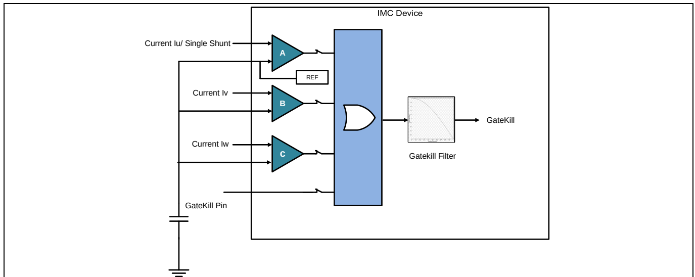
Figure 13 Overcurrent Protection Internal Comparator
