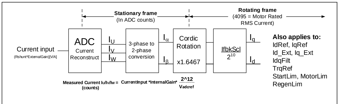
Figure 6 Motor current feedback signal path
