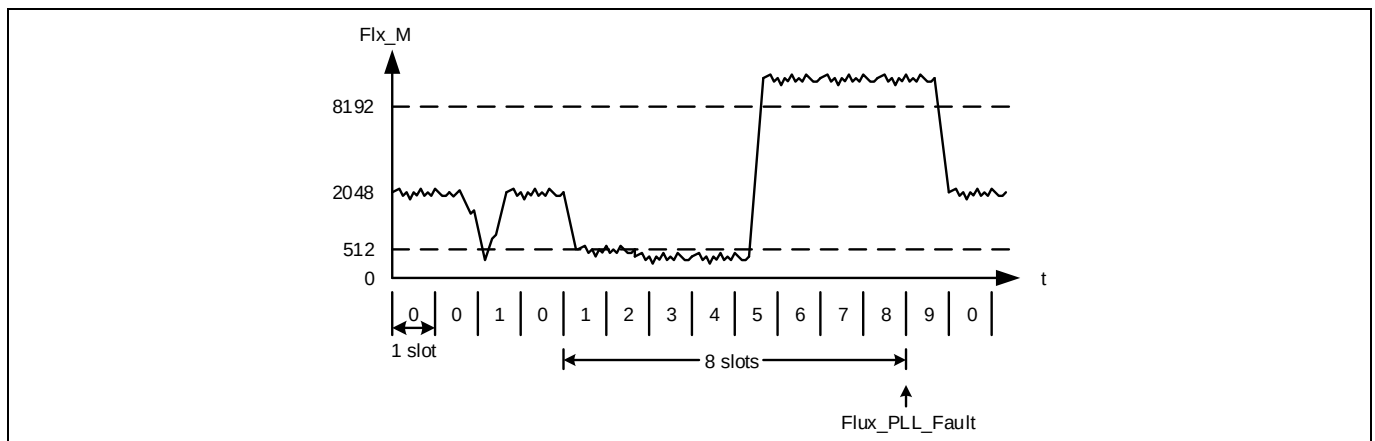
Figure 12 Flux PLL out-of-control protection
