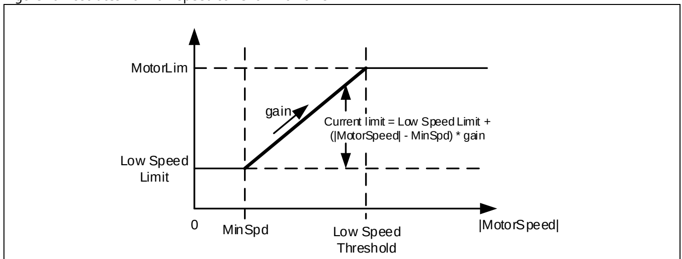
Figure 10 Low speed current limit (Motoring limit)
