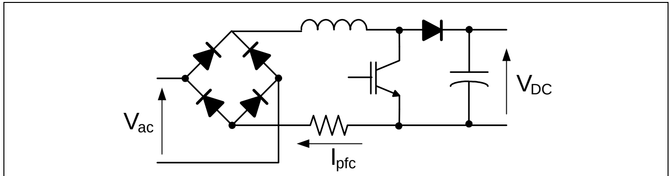
Figure 23 Basic Boost PFC Circuit
