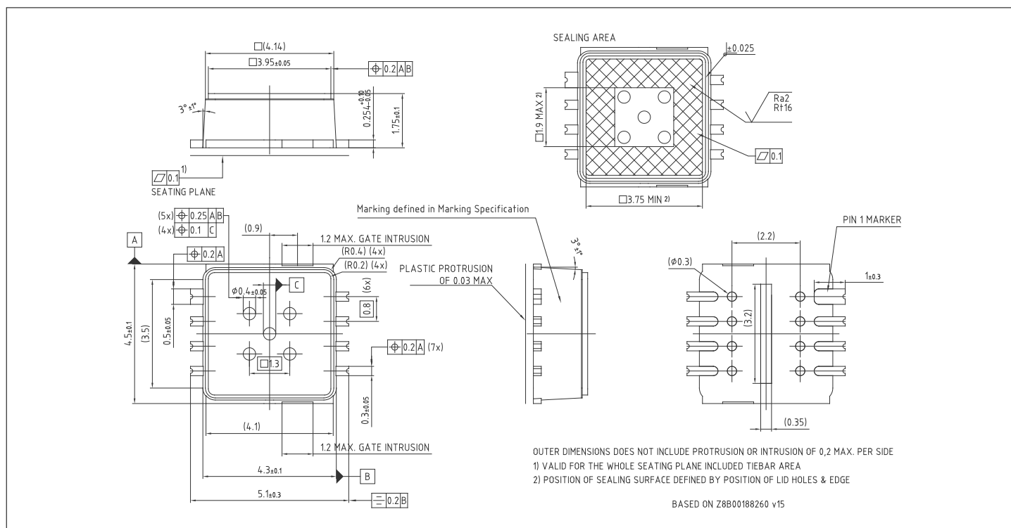
Figure 41 PG-DFN-8-1 outlines
