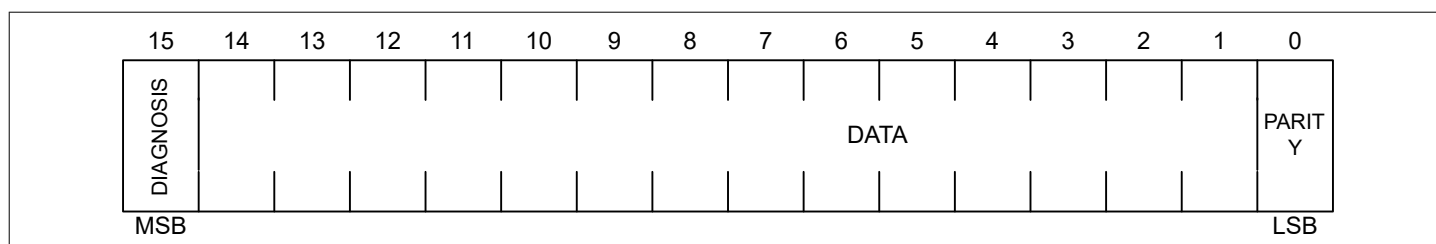
Figure 10 SPI response structure (14-bit)
