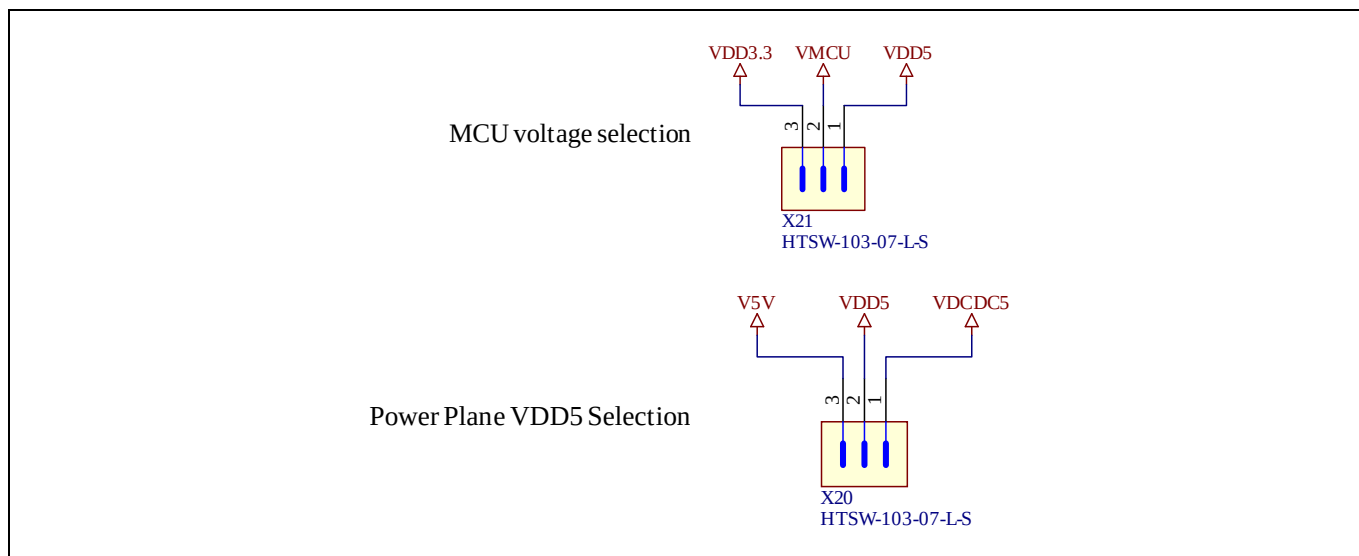
Figure 39 XMC7200 VDDIO2 voltage selection
