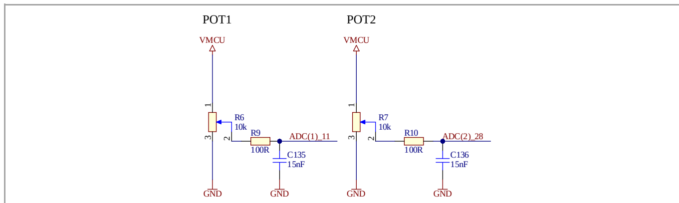
Figure 33 Potentiometers
