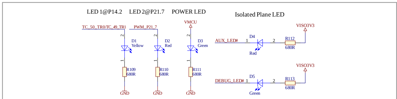
Figure 30 User LEDs
