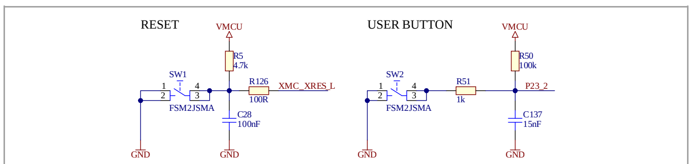
Figure 31 User buttons
