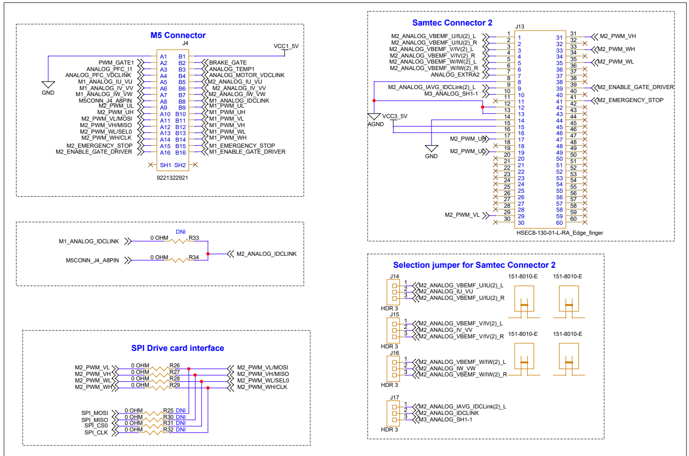
Figure 27 M5 connector and Samtec connector 2
