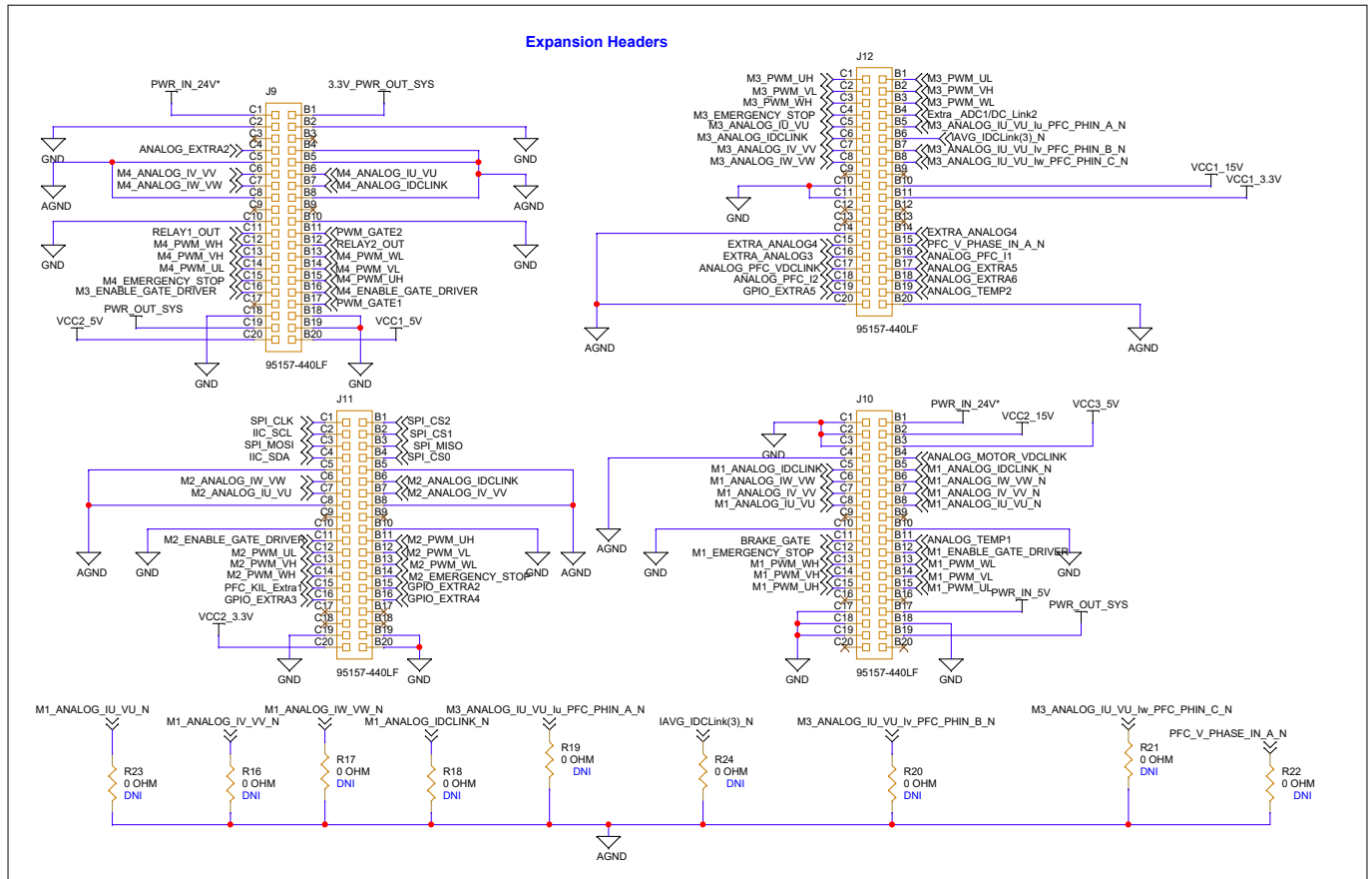
Figure 28 Drive adapter card expansion headers
