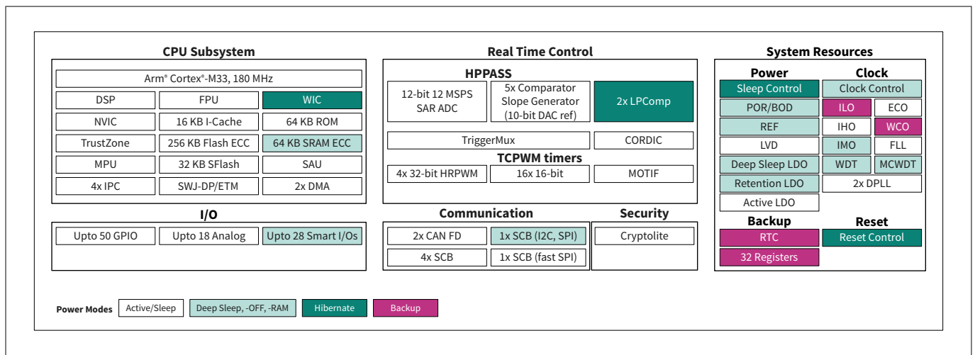
Figure 12 PSOC™ Control C3M5 MCU block diagram
