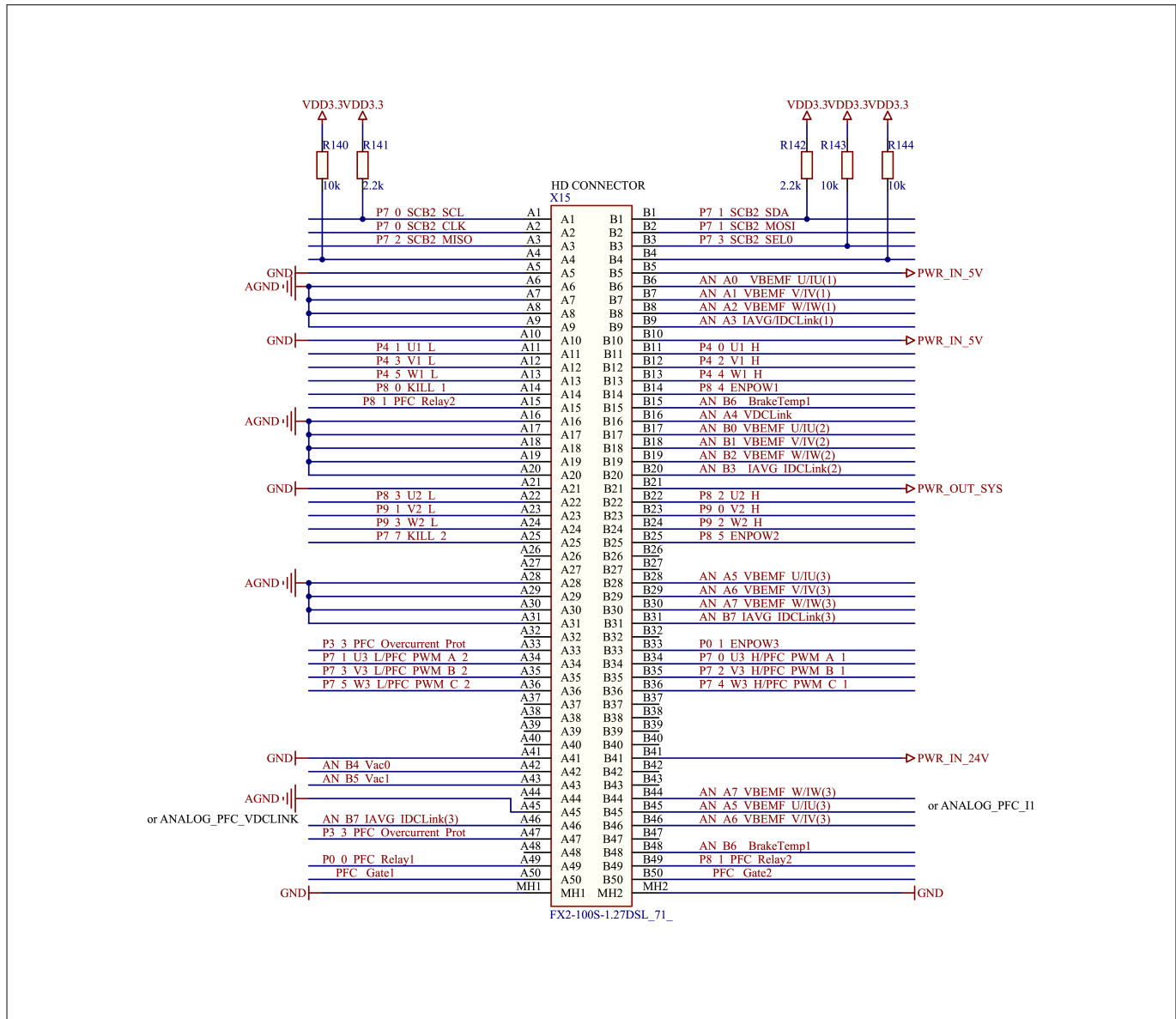
Figure 16 100-pin HD connector
