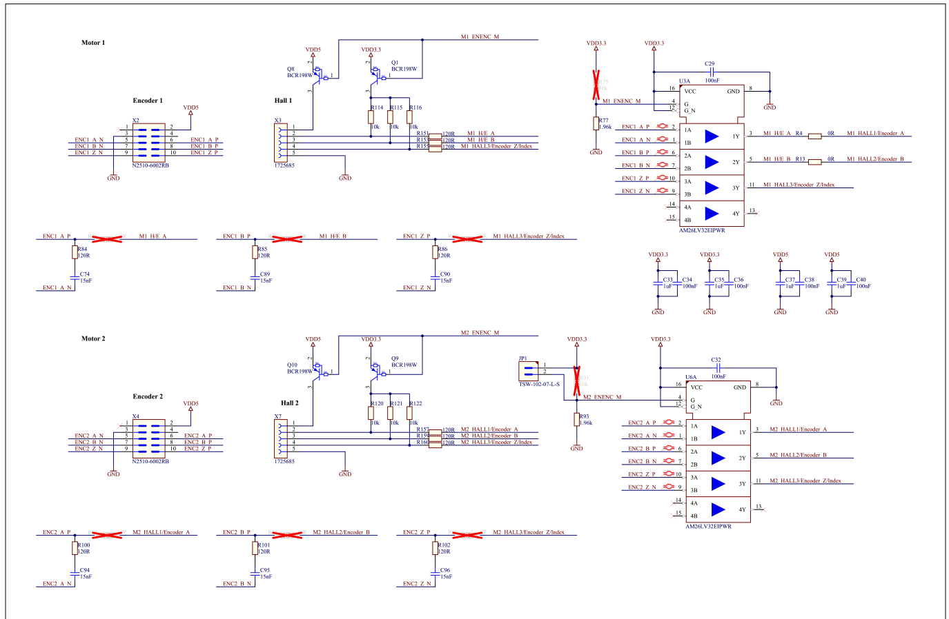
Figure 24 Hall sensor and encoder interface
