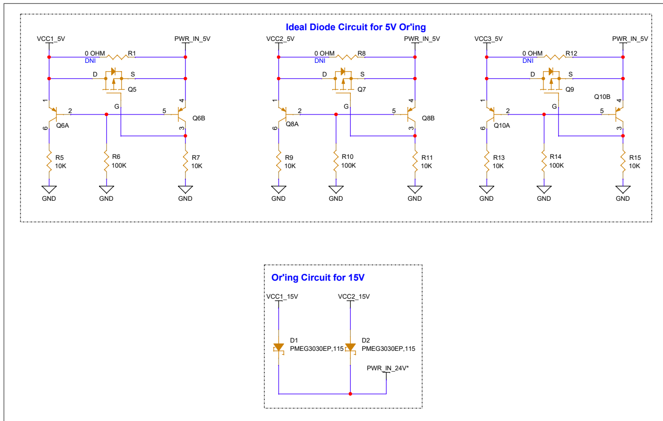
Figure 29 Power supply ORing circuits
