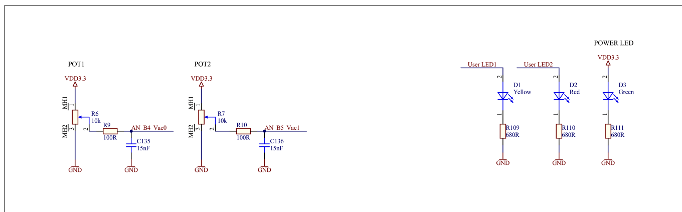
Figure 19 Potentiometers and user LEDs
