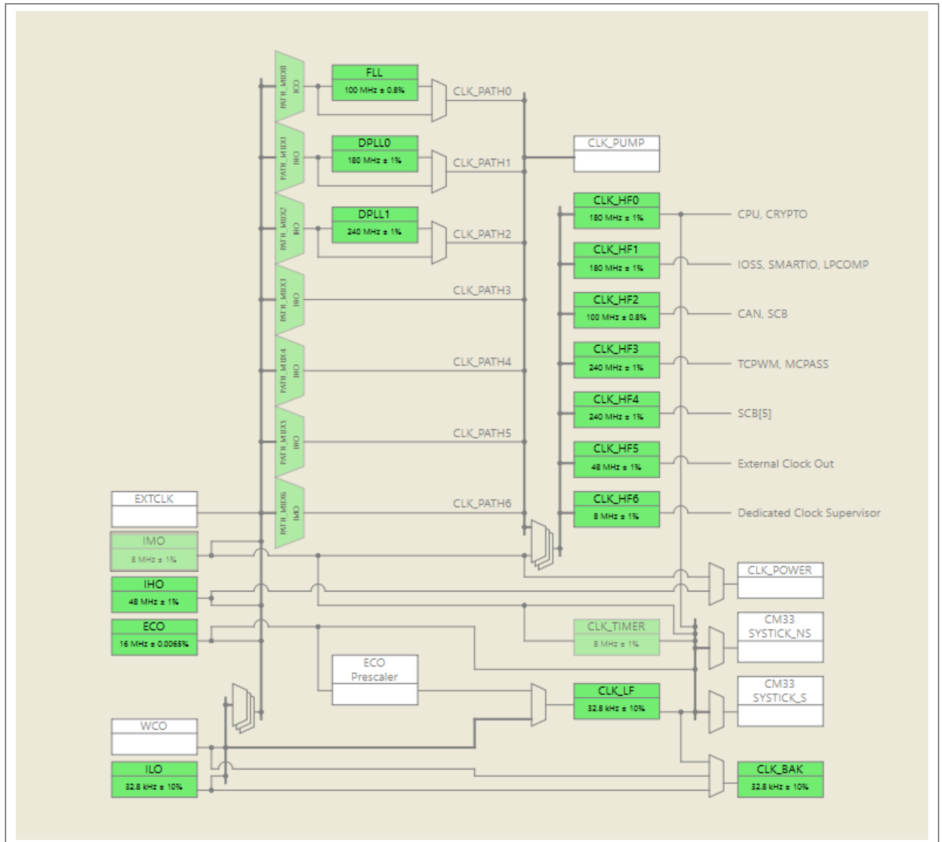
Figure 21 PSOC™ Control C3 MCU clock architecture
