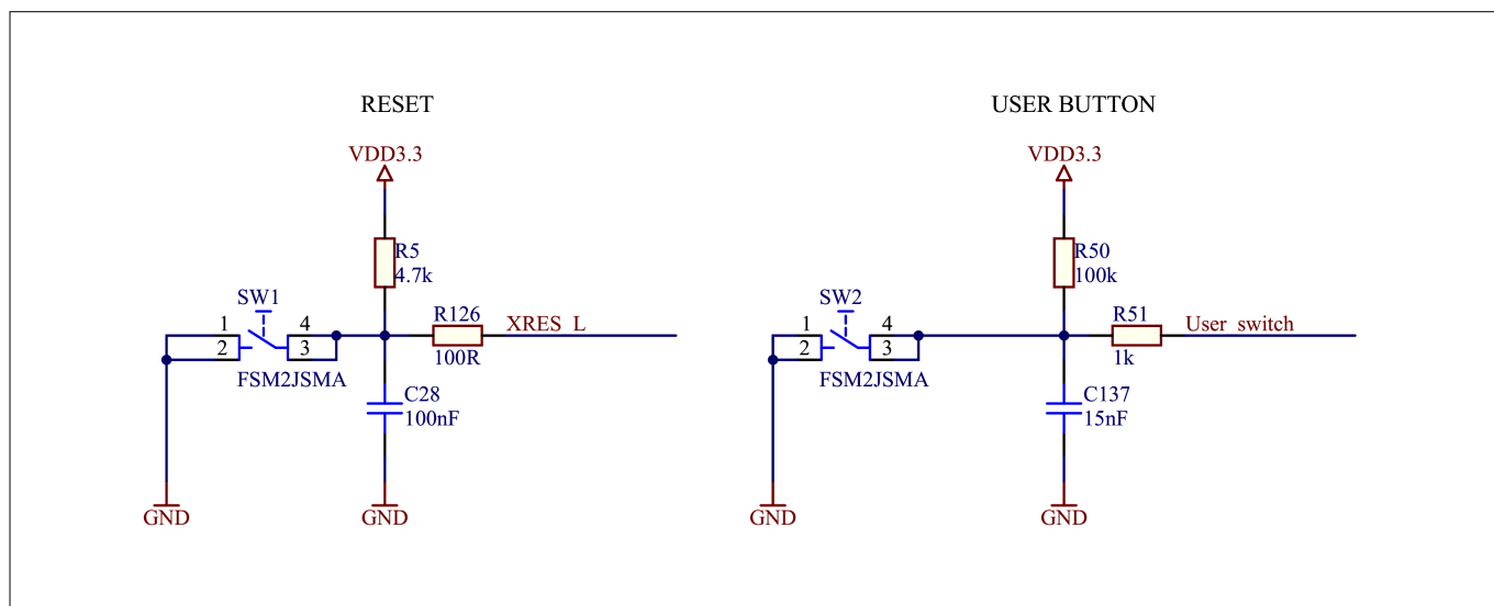
Figure 18 Reset and user buttons
