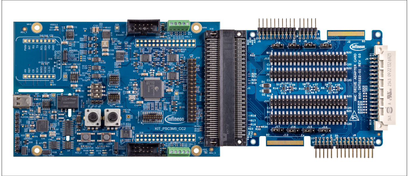
Figure 4 KIT_PSC3M5_CC2 motor control card connected to the drive adapter card
