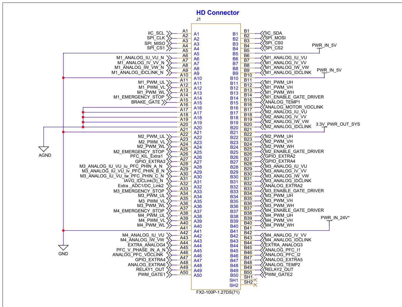
Figure 25 Drive adapter card 100-pin HD connector
