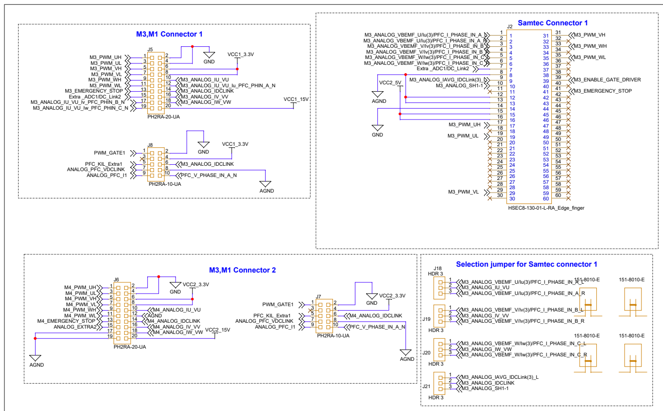
Figure 26 M3, M1 connectors and Samtec connector 1
