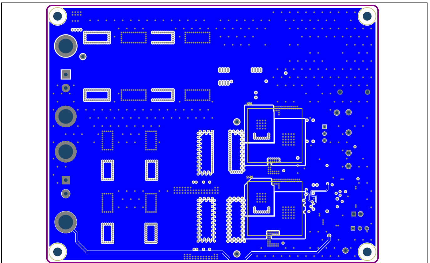
Figure 15 Bottom overlay
