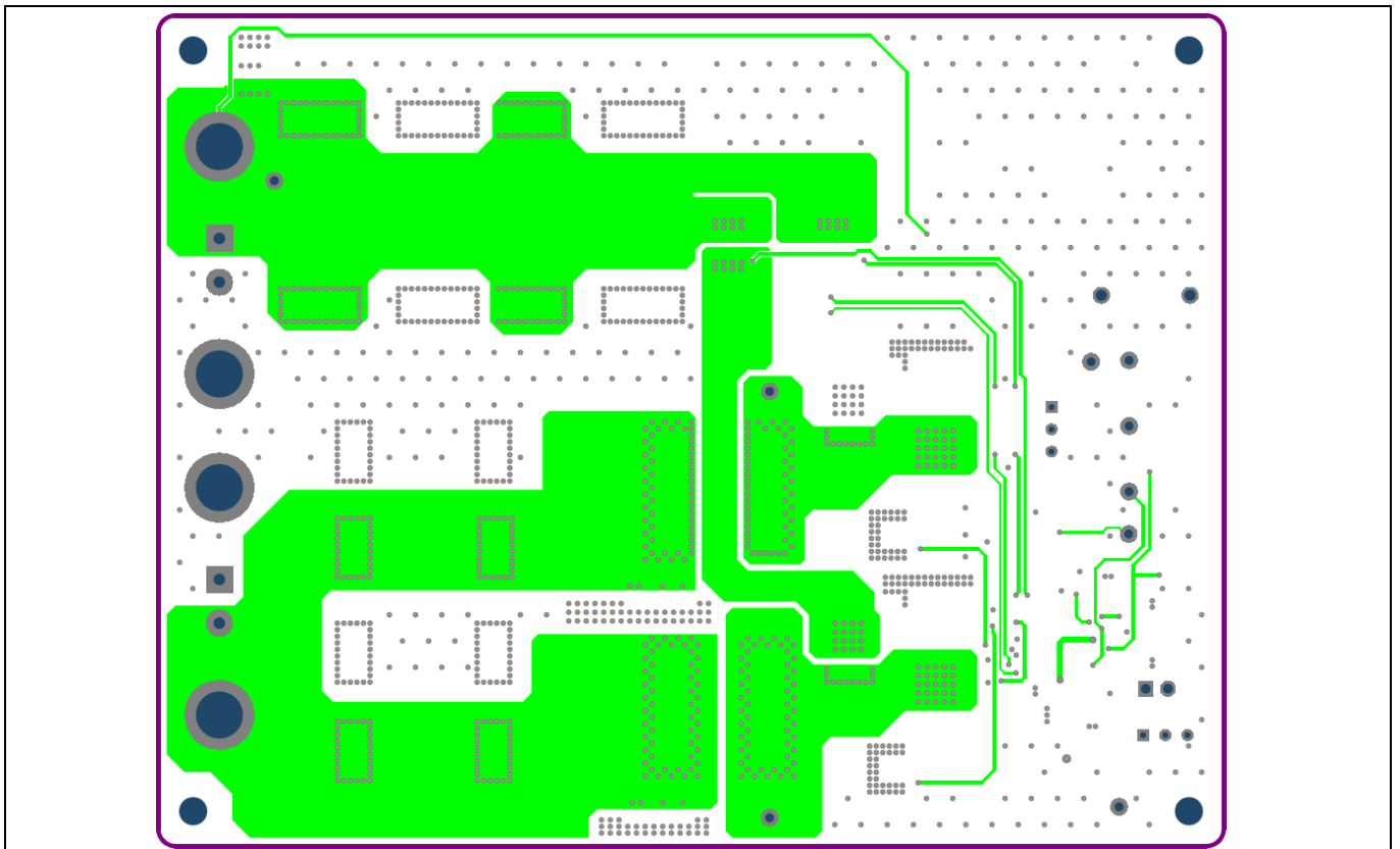
Figure 14 Internal overlay 2
