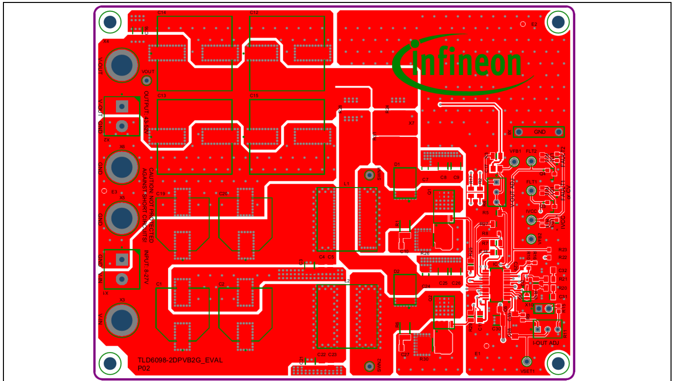
Figure 12 Top overlay
