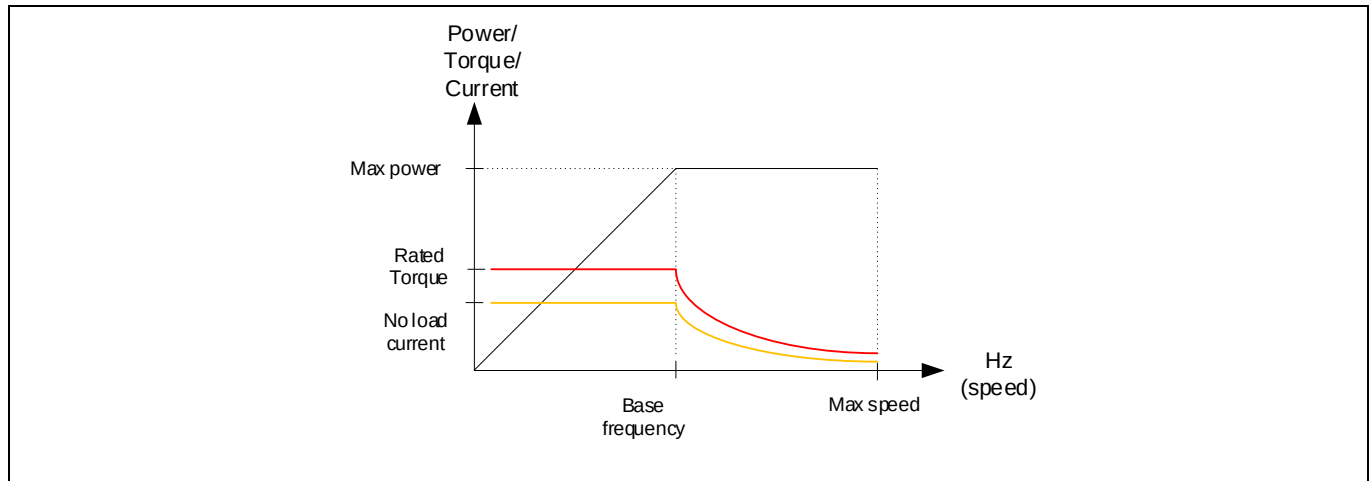
Figure 9 Field weakening
