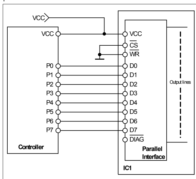
Figure 10 Parallel Direct Control
