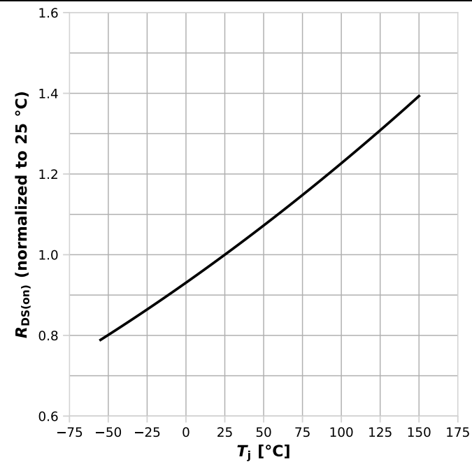
Diagram 24: Normalized drain-source on resistance (p-ch.)
