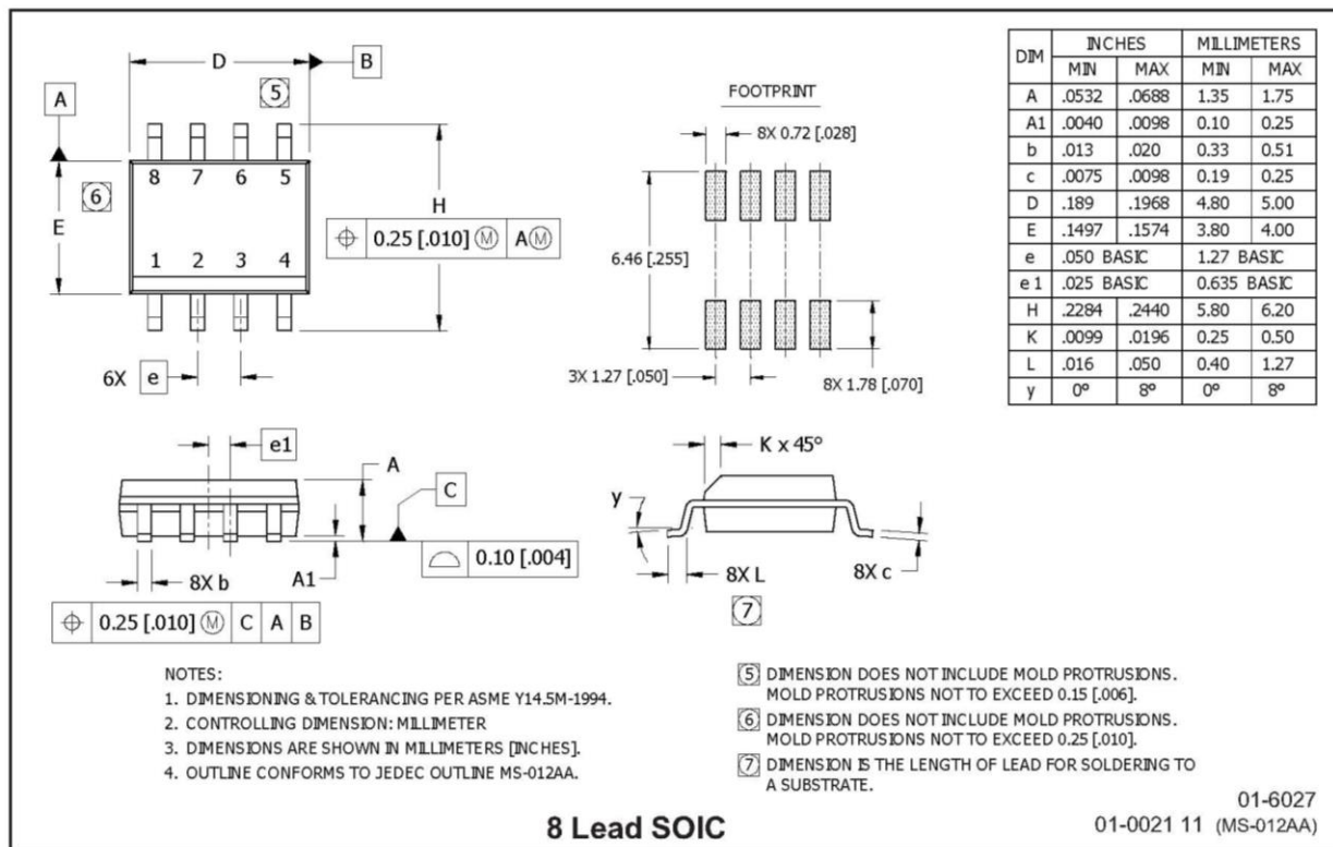
Figure 12 Package details
