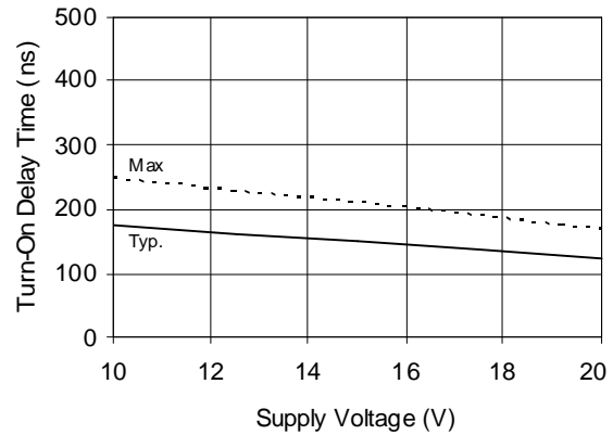
Figure 17B. Turn-On Propagation Delay vs. Supply Voltage
