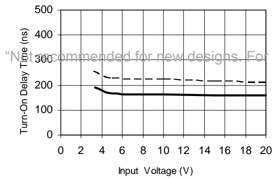
Figure 6C. Turn-On Time vs. Input Voltage
