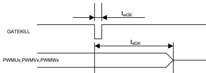
Figure 10. Gatekill timing
