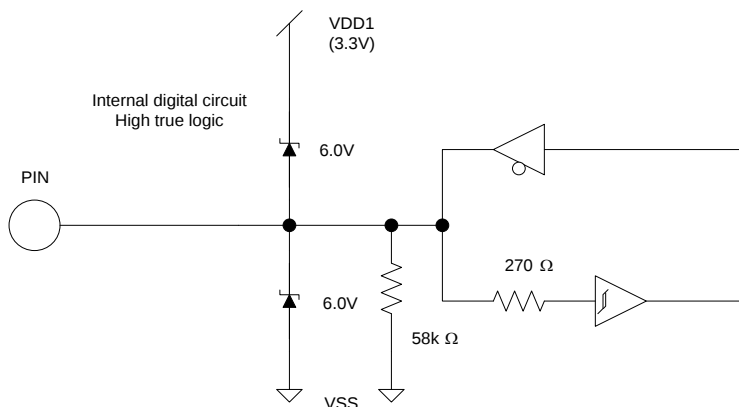
Figure 19. PWMUL/PWMUH/PWMVL/PWMVH/PWMWL/PWMWH output
