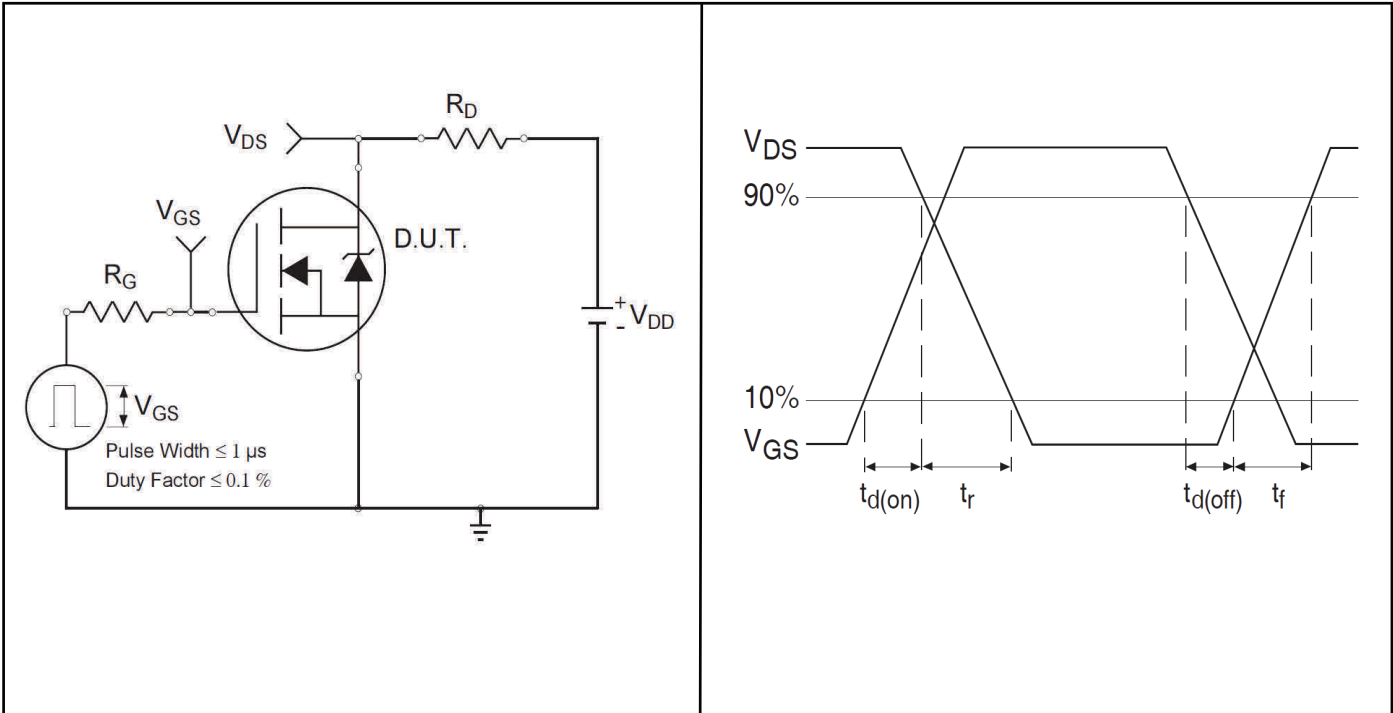
Figure 13b Switching Time Waveforms
