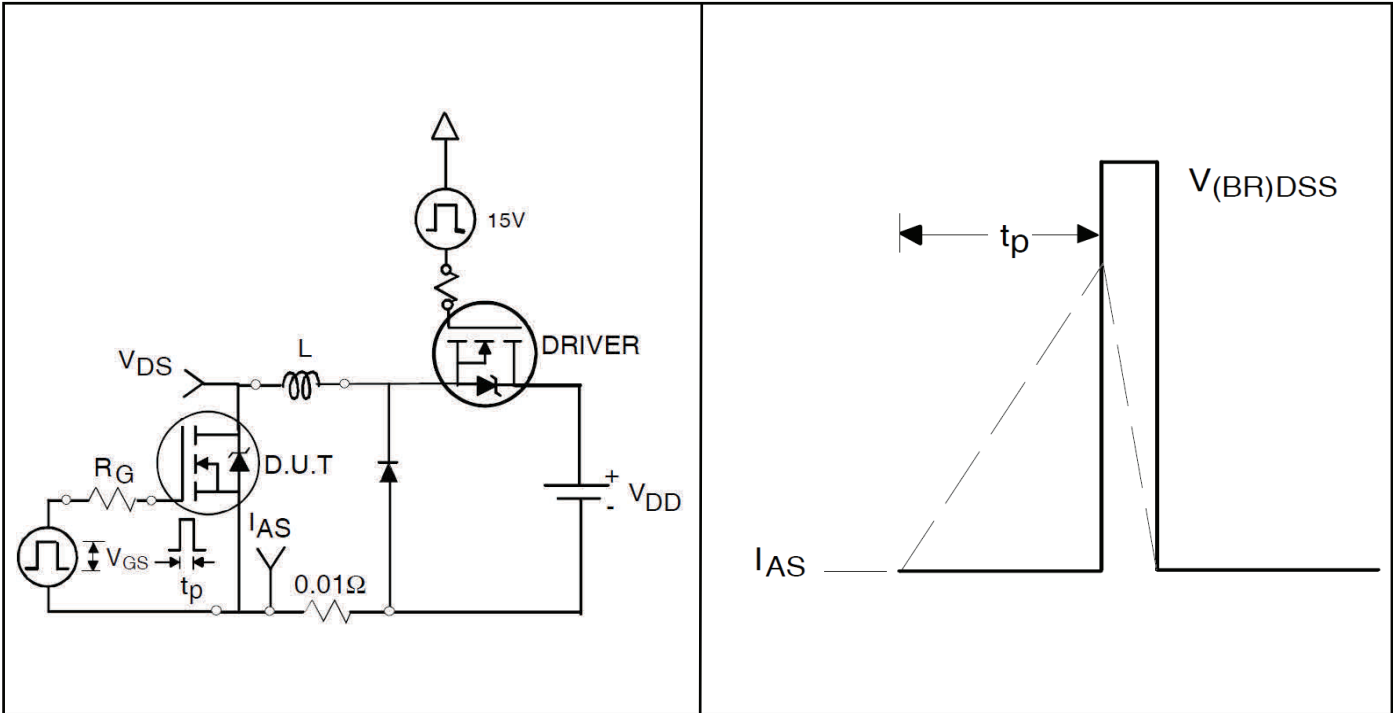
Figure 15b Unclamped Inductive Waveforms
