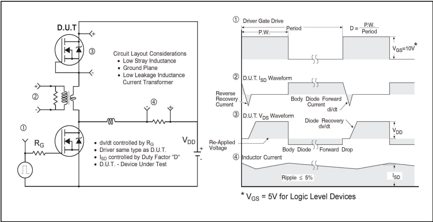
Figure 14 Peak Diode Recovery dv/dt Test Circuit for N-Channel HEXFET™ Power MOSFETs
