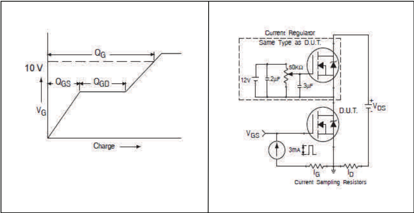
Figure 16b Gate Charge Test Circuit
