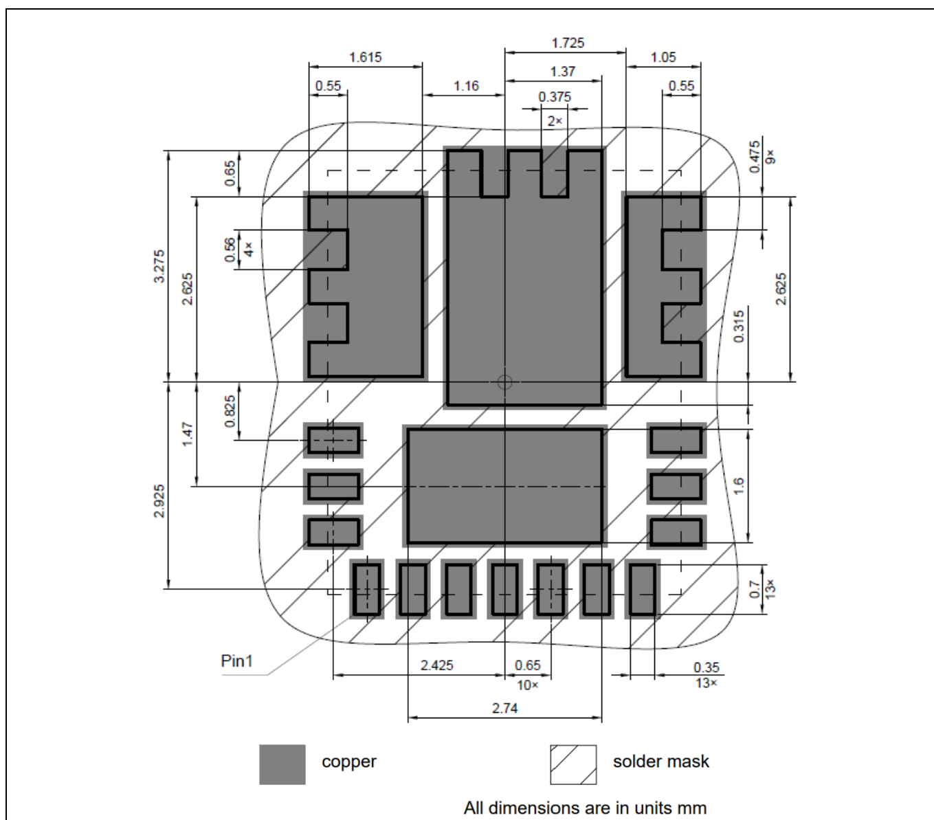
Figure 30 Solder mask (all dimensions in mm)
