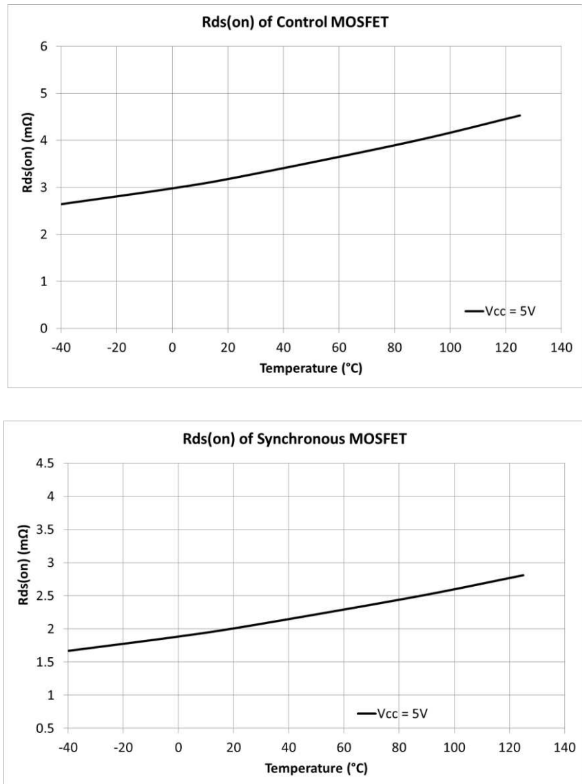
Figure 5 R DS(on) of MOSFETs over Junction Temperature
