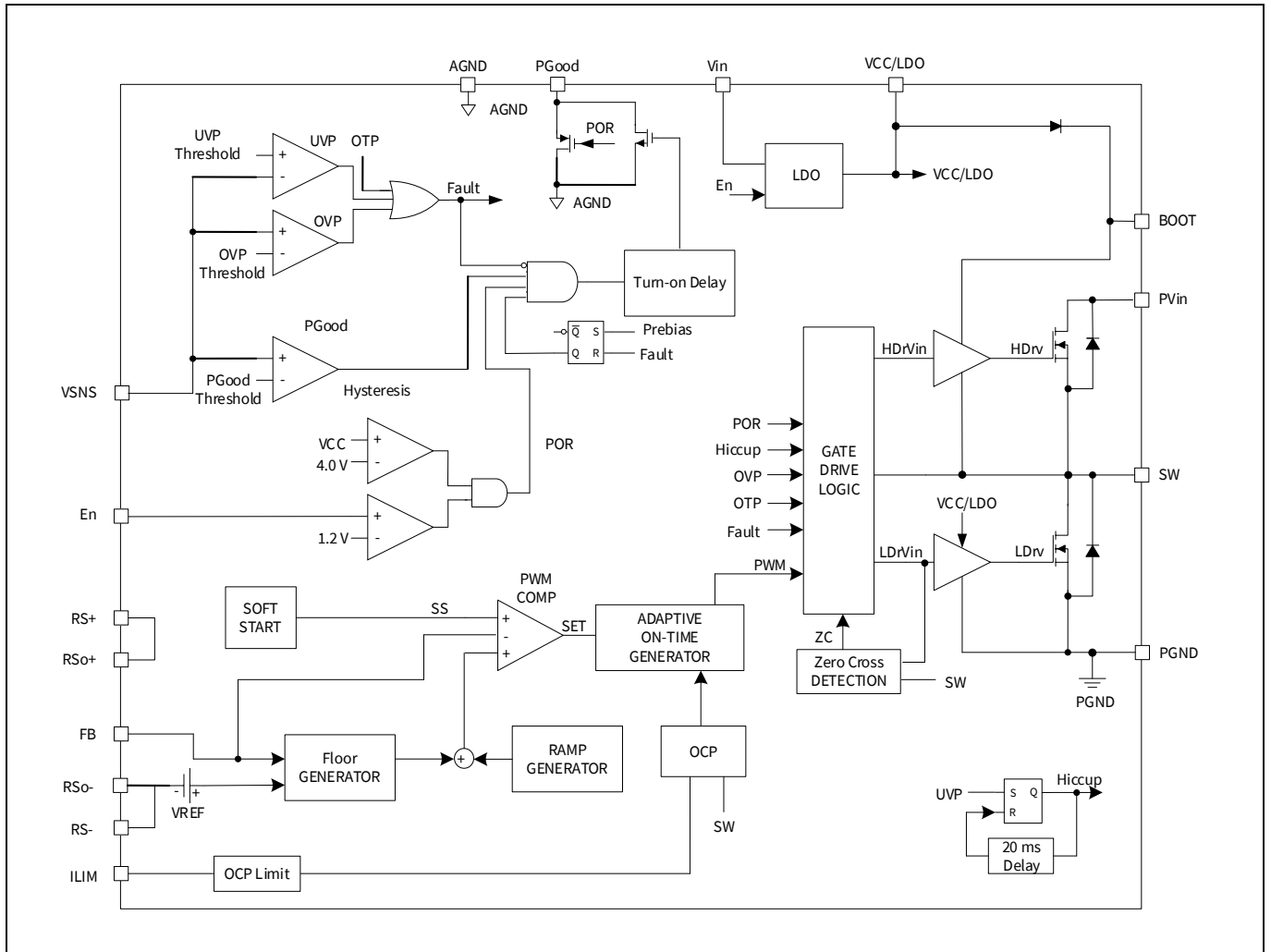
Figure 2 Block diagram
