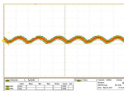
Output voltage ripple, 23 A load Ch1: V_{out} , peak-to-peak V_{out-ripple} = 11.6\text{ mV}
