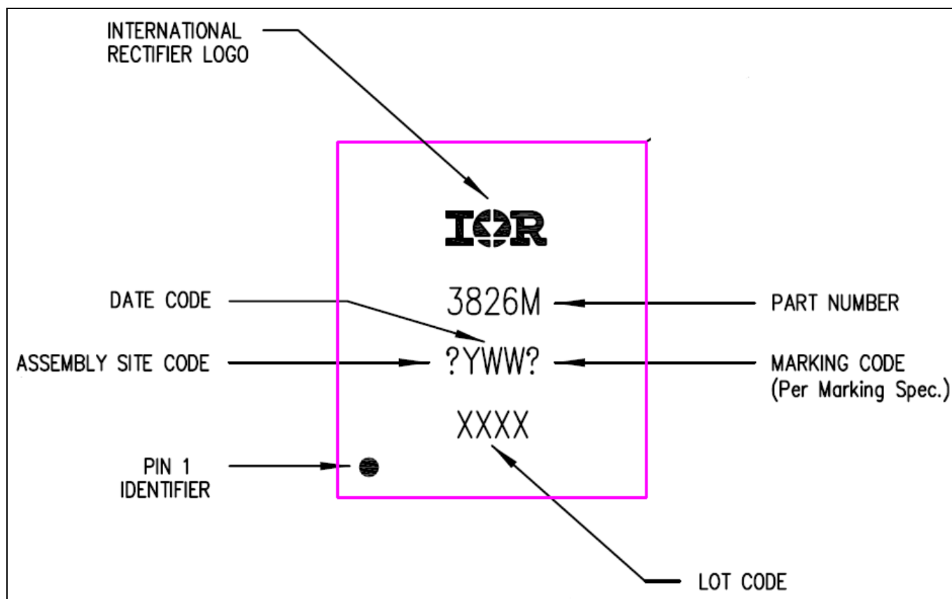
Figure 36 Package Marking
