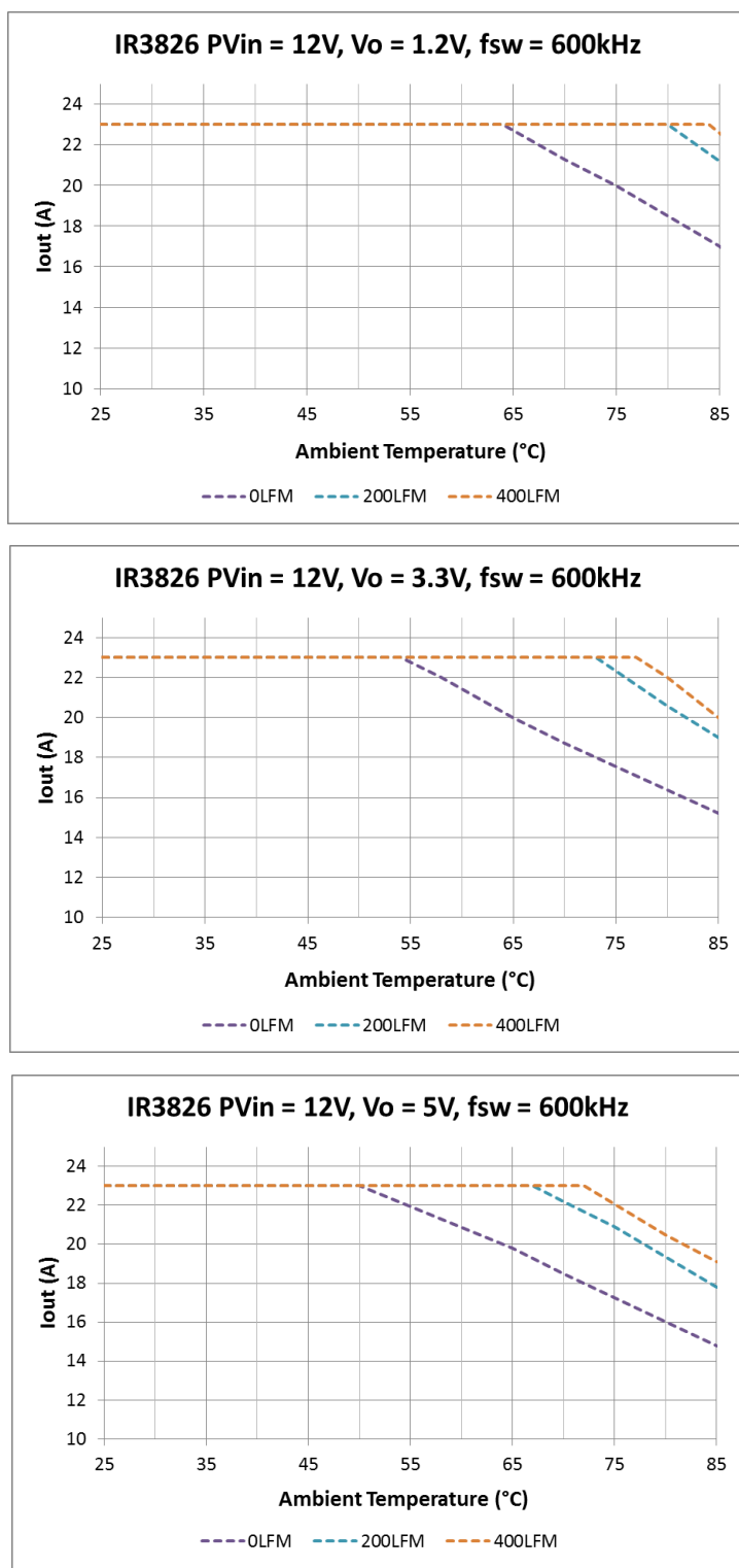
Figure 4 Thermal derating curves, P_{Vin} = 12V , V_{out} = 1.2V/3.3V/5V , V_{cc} = \text{Internal LDO} , F_s = 600kHz
