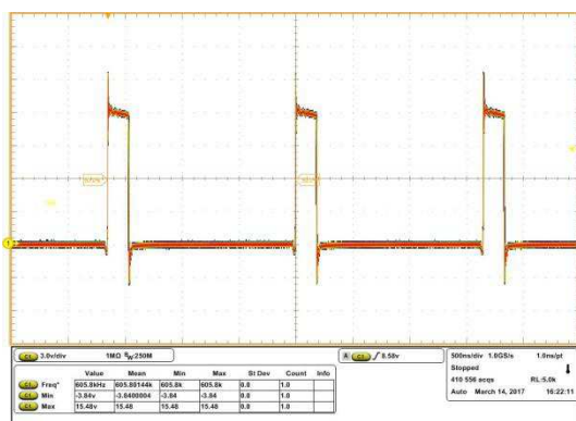
Inductor node at 23 A load Ch1: Switch Node
