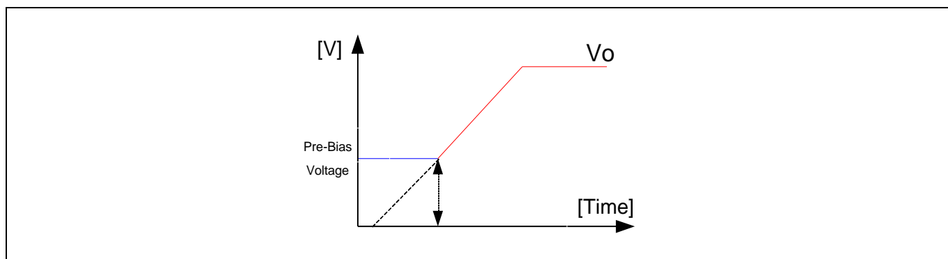
Figure 17 Pre-Bias startup
