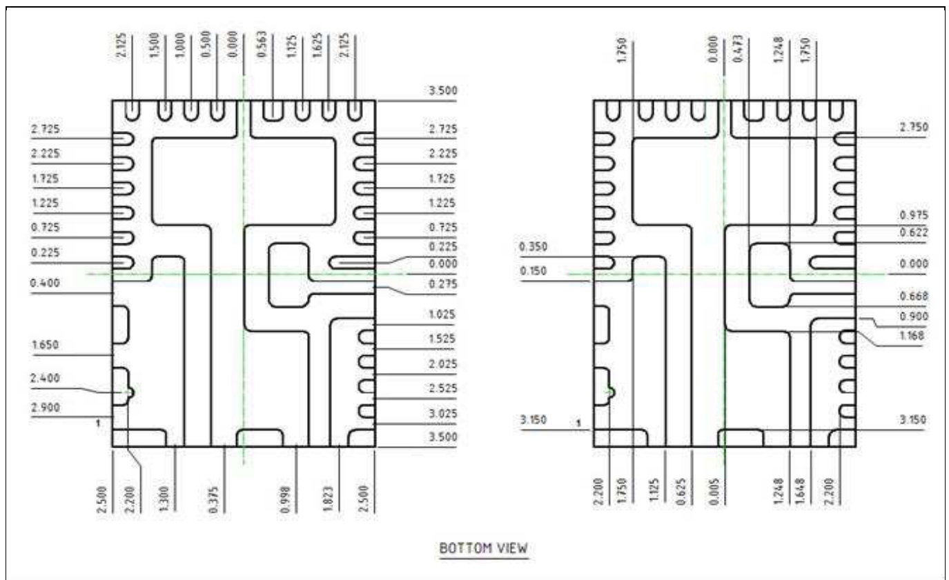
Figure 47 Package dimensions
