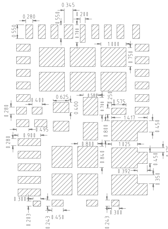
Figure 41 Solder paste stencil (pad sizes)
