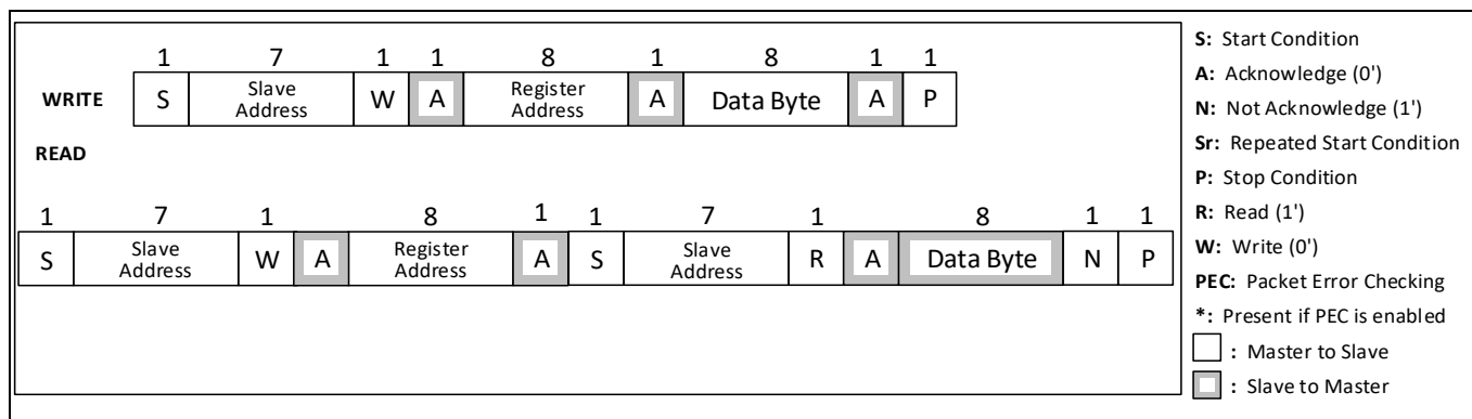
Figure 30 I2C format
