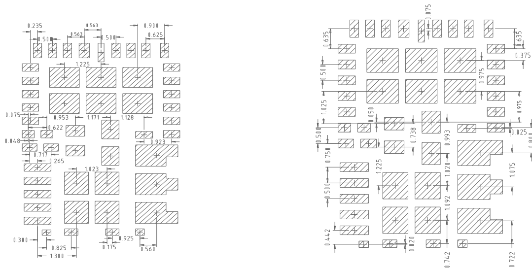
Figure 42 Solder paste stencil (pad spacing)
