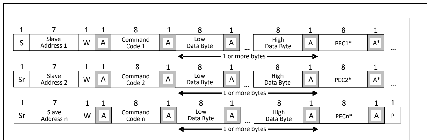
Figure 37 Group command
