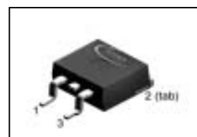
PG-TO263-3-2
