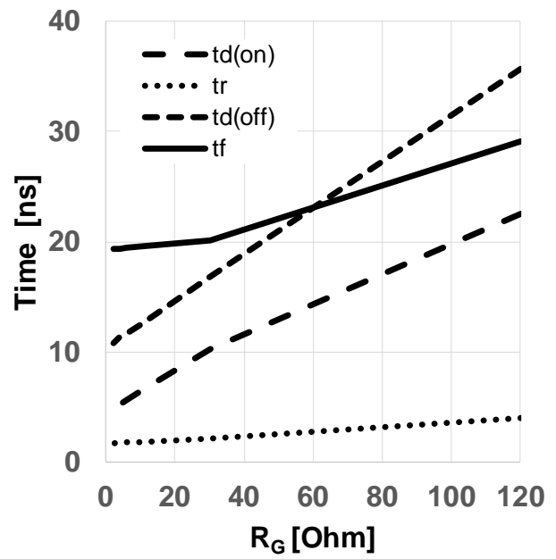
Figure 18 Typical switching times as a function of gate resistor (t = f(R_{G,ext}), V_{DD} = 800V, V_{GS} = 0V/18V, I_D = 2A, T_{vj} = 175^{\circ}C, \text{ind. load, test circuit in} Fig. E, diode: body diode at V_{GS} = 0V)
