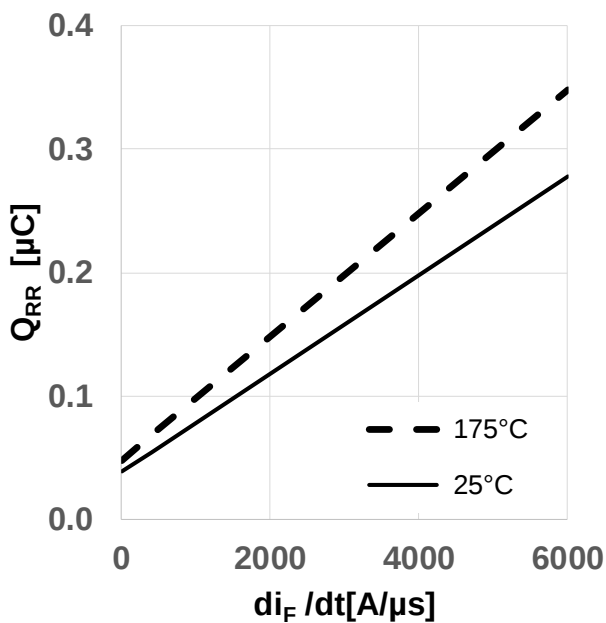
Figure 19 Typical reverse recovery charge as a function of diode current slope (Q_{rr} = f(di_F/dt), V_{DD} = 800V, V_{GS} = 0V/18V, I_D = 4A, \text{ind. load, test circuit in Fig. E, body diode at } V_{GS} = 0V)
