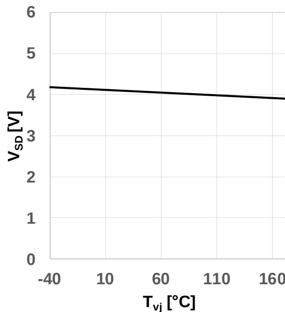
Figure 12 Typical body diode forward voltage as function of junction temperature ( V_{SD} = f(T_{vj}) , V_{GS} = 0V , I_{SD} = 13A )
