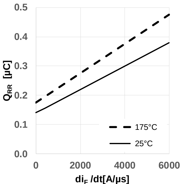
Figure 19 Typical reverse recovery charge as a function of diode current slope (Q_{rr} = f(di_i/dt), V_{DD} = 800V, V_{GS} = 0V/18V, I_D = 13A, \text{ind. load, test circuit in Fig.E,} body diode at V_{GS} = 0V)
