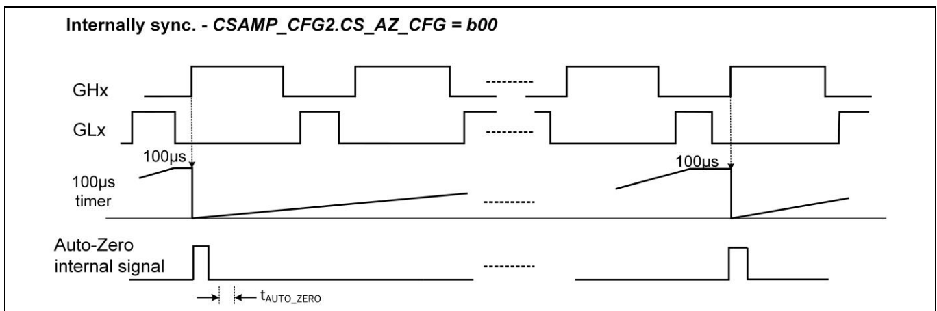
Figure 47 Auto-Zero operating modes. Auto-Zero occurs upon next GHx rising edge after timer has reached 100μs. Auto-Zero period will then rest the timer again
