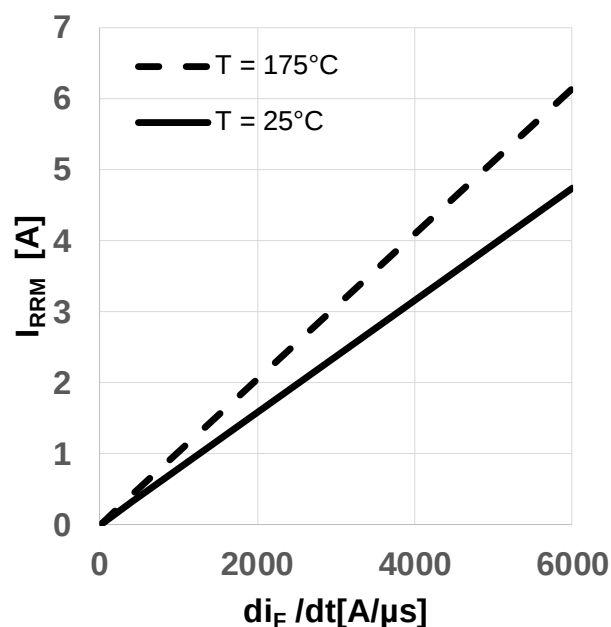
Figure 20 Typical reverse recovery current as a function of diode current slope (I_{rrm} = f(di_i/dt), V_{DD} = 800V, V_{GS} = 0V/18V, I_D = 4A, \text{ind. load, test circuit in Fig. E, body diode at } V_{GS} = 0V)
