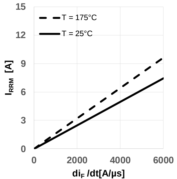
Figure 20 Typical reverse recovery current as a function of diode current slope (I_{rrm} = f(di_t/dt), V_{DD} = 800V, V_{GS} = 0V/18V, I_D = 6A, \text{ind. load, test circuit in Fig. E, body diode at } V_{GS} = 0V)
