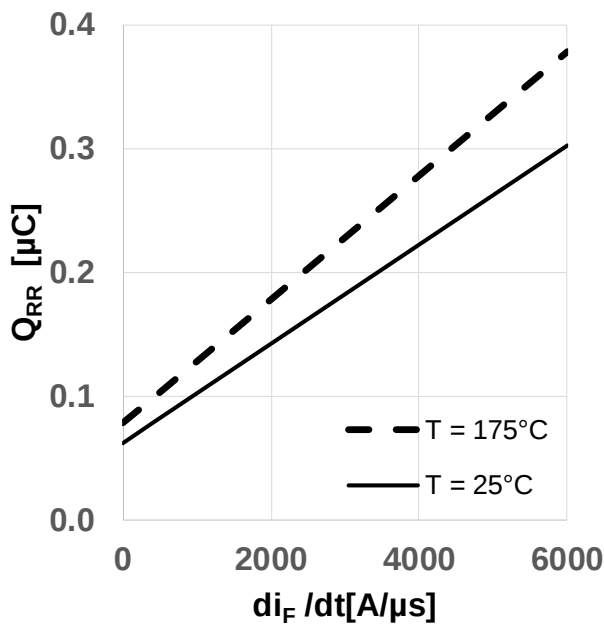
Figure 19 Typical reverse recovery charge as a function of diode current slope (Q_{rr} = f(di_t/dt), V_{DD} = 800V, V_{GS} = 0V/18V, I_D = 6A, \text{ind. load, test circuit in Fig. E, body diode at } V_{GS} = 0V)
