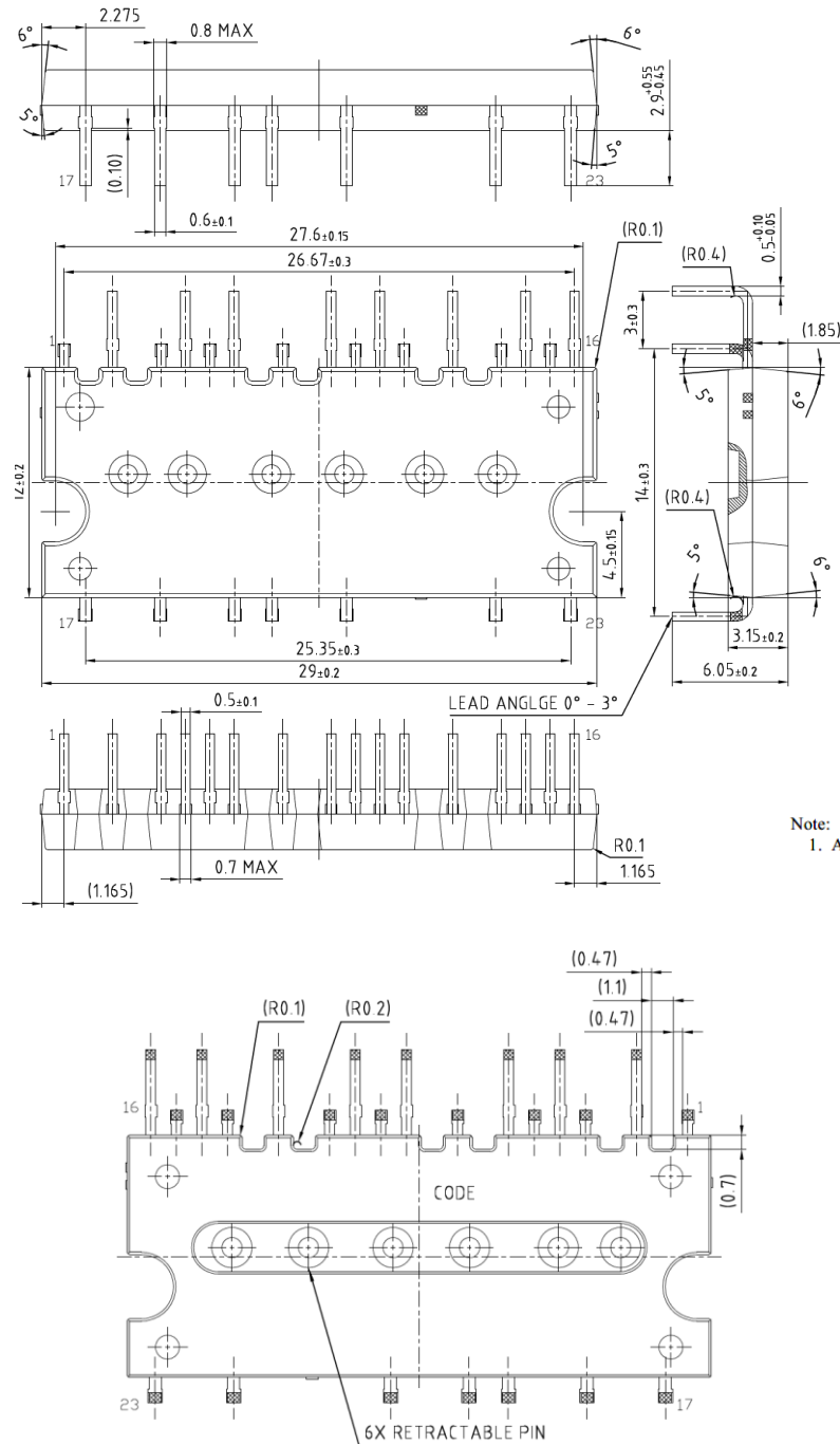
Figure 16 IM241-S6T2x (DIP 29x12)
