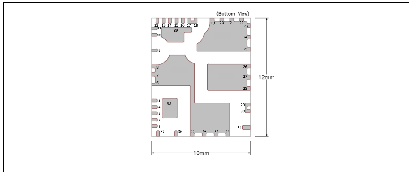
Figure 2 Module pinout
