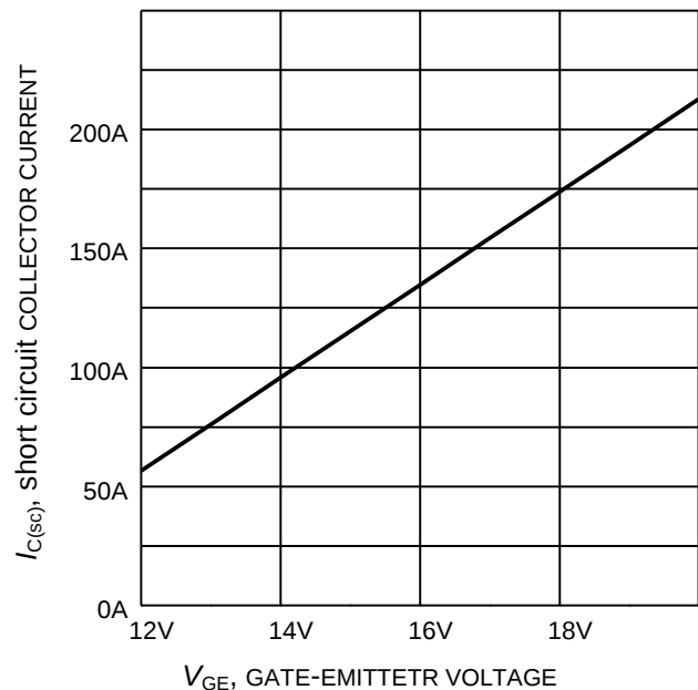
Figure 20. Typical short circuit collector current as a function of gate-emittetr voltage ( V_{CE} \leq 600\text{ V} , T_{j,\text{start}} = 175^\circ\text{C} )
