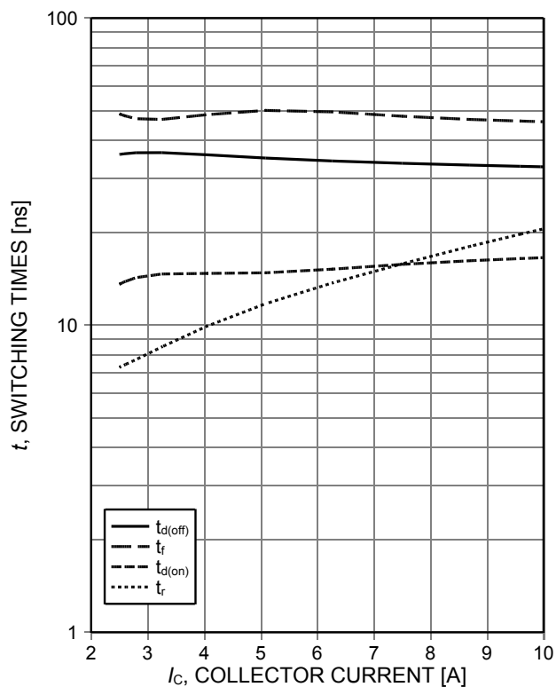
Figure 8. Typical switching times as a function of collector current (inductive load, T_{vj} = 150^\circ\text{C} , V_{CE} = 400\text{V} , V_{GE} = 0/15\text{V} , R_G = 47\Omega , Dynamic test circuit in Figure E)
