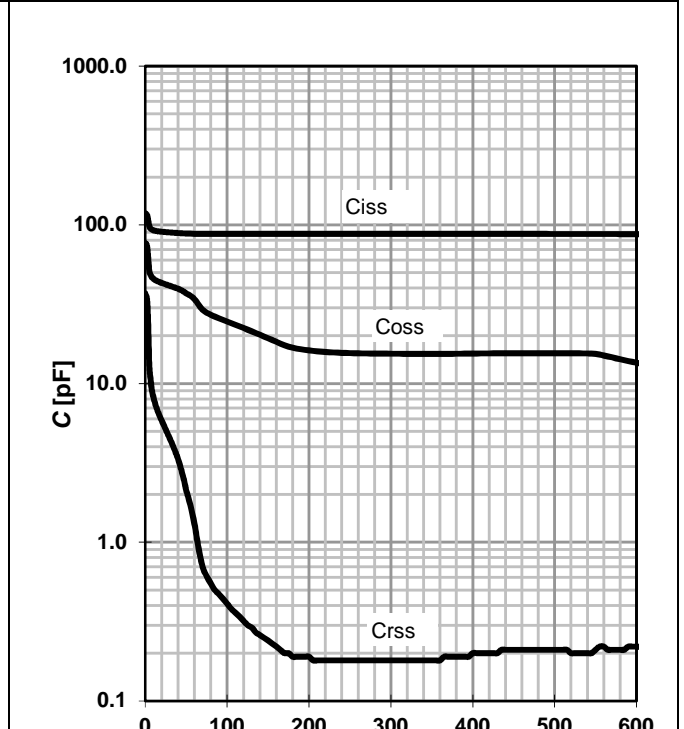
Figure 20 Typ. capacitances
