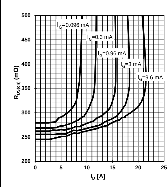
Figure 9 Typ. Drain-source on-state resistance
