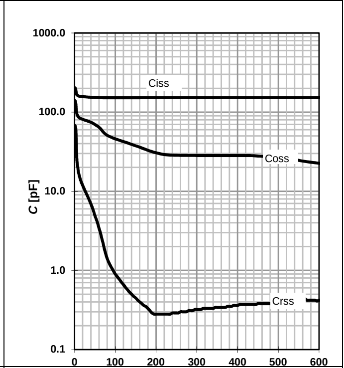
Figure 20 Typ. capacitances
