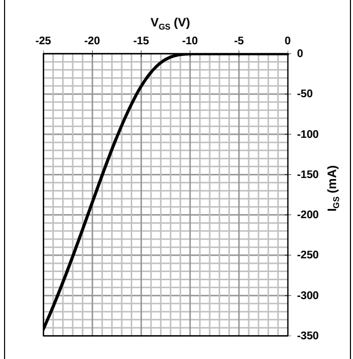
Figure 12 Typ. gate characteristics reverse
